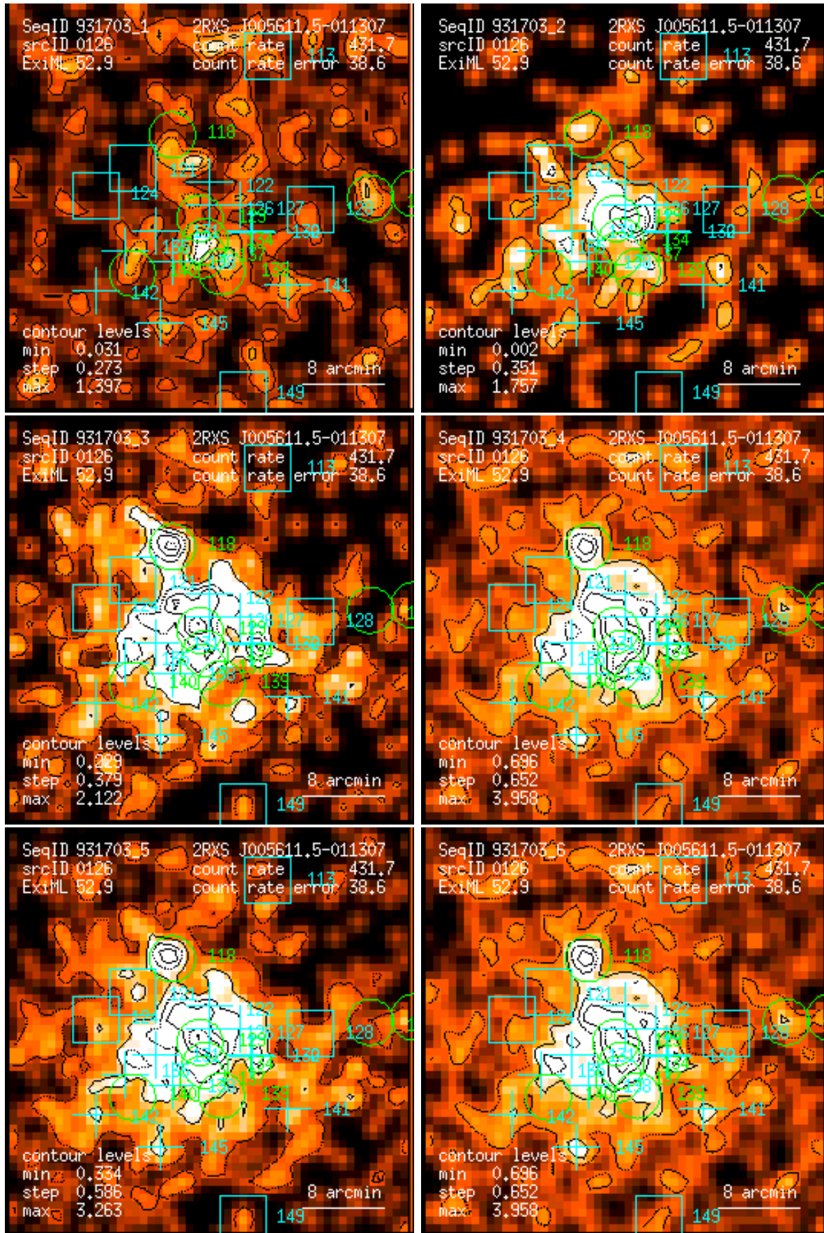
Figure 126: RASS 931703: detection 0126: band rate images, Gaussian filter: (1) PSPC channels 11 – 41, (2) 52 – 90, (3) 91 – 201, (4) 11 – 235, (5) 52 – 201, (6) 11 – 201. Broad band rates in counts/ks. Band rate contour levels in counts/ks/arcmin 2 .
