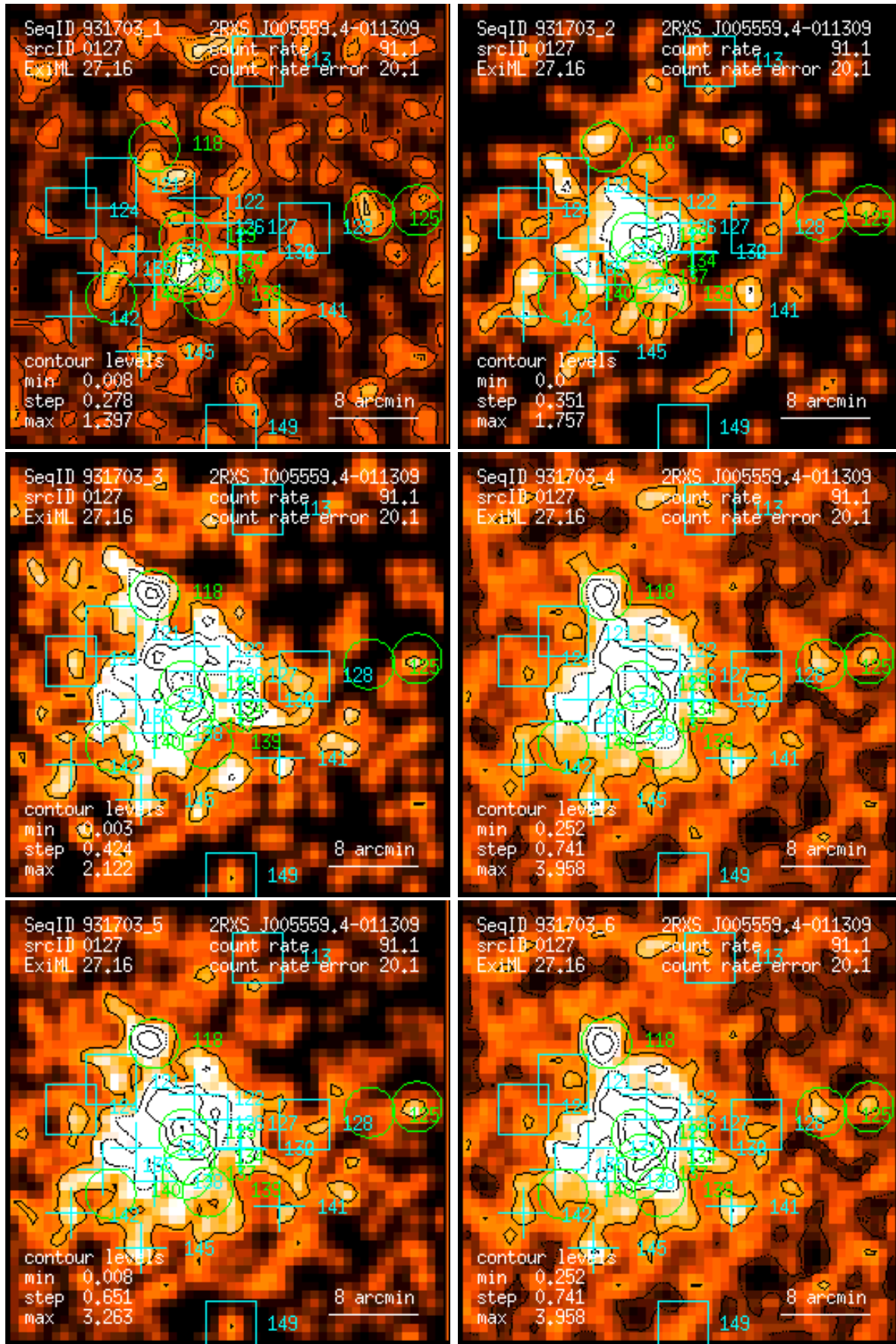
Figure 127: RASS 931703: detection 0127: band rate images, Gaussian filter: (1) PSPC channels 11 – 41, (2) 52 – 90, (3) 91 – 201, (4) 11 – 235, (5) 52 – 201, (6) 11 – 201. Broad band rates in counts/ks. Band rate contour levels in counts/ks/arcmin 2 .
