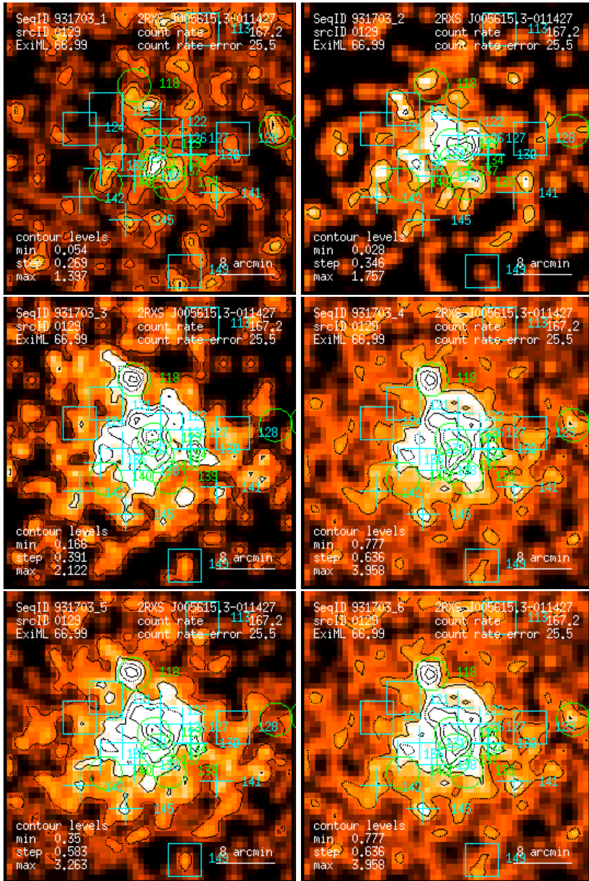
Figure 129: RASS 931703: detection 0129: band rate images, Gaussian filter: (1) PSPC channels 11 – 41, (2) 52 – 90, (3) 91 – 201, (4) 11 – 235, (5) 52 – 201, (6) 11 – 201. Broad band rates in counts/ks. Band rate contour levels in counts/ks/arcmin 2 .
