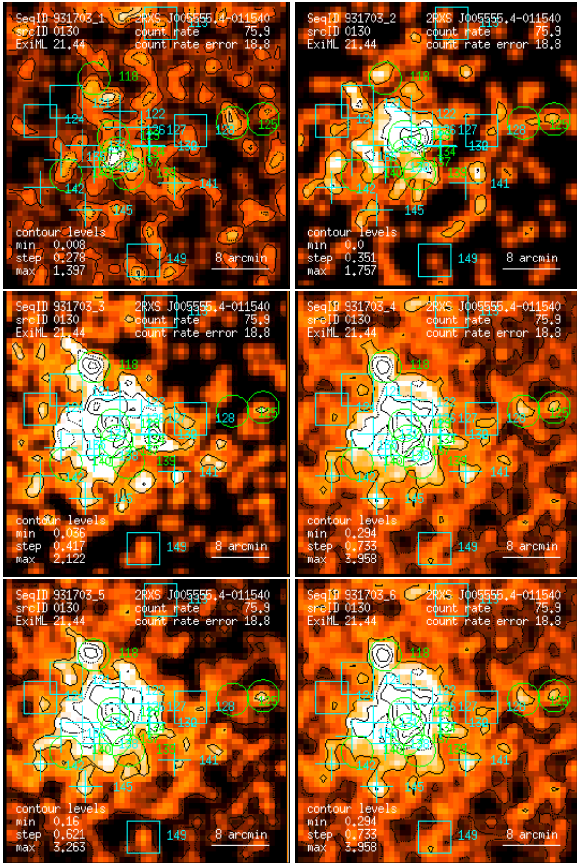
Figure 130: RASS 931703: detection 0130: band rate images, Gaussian filter: (1) PSPC channels 11 – 41, (2) 52 – 90, (3) 91 – 201, (4) 11 – 235, (5) 52 – 201, (6) 11 – 201. Broad band rates in counts/ks. Band rate contour levels in counts/ks/arcmin 2 .
