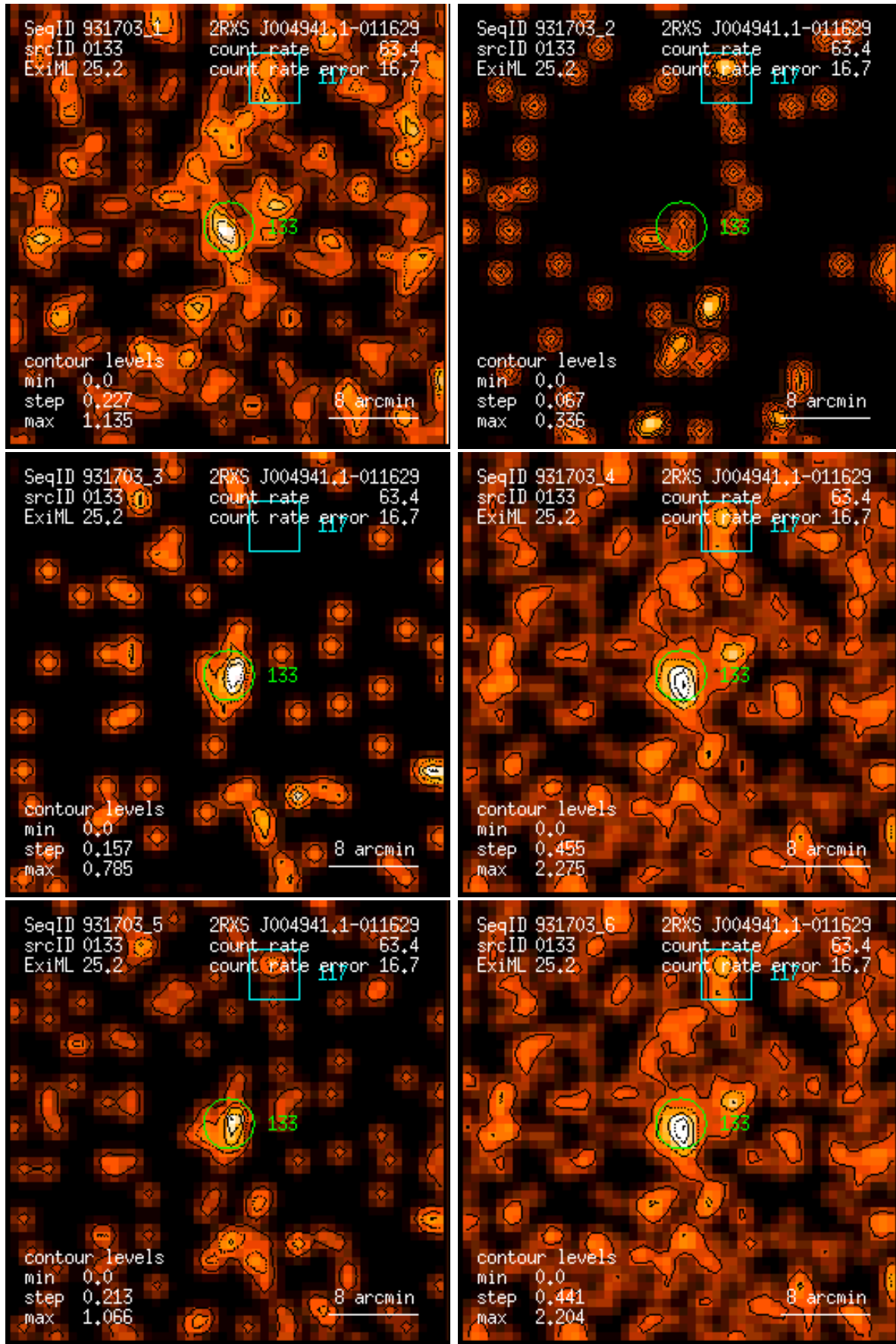
Figure 133: RASS 931703: detection 0133: band rate images, Gaussian filter: (1) PSPC channels 11 – 41, (2) 52 – 90, (3) 91 – 201, (4) 11 – 235, (5) 52 – 201, (6) 11 – 201. Broad band rates in counts/ks. Band rate contour levels in counts/ks/arcmin 2 .
