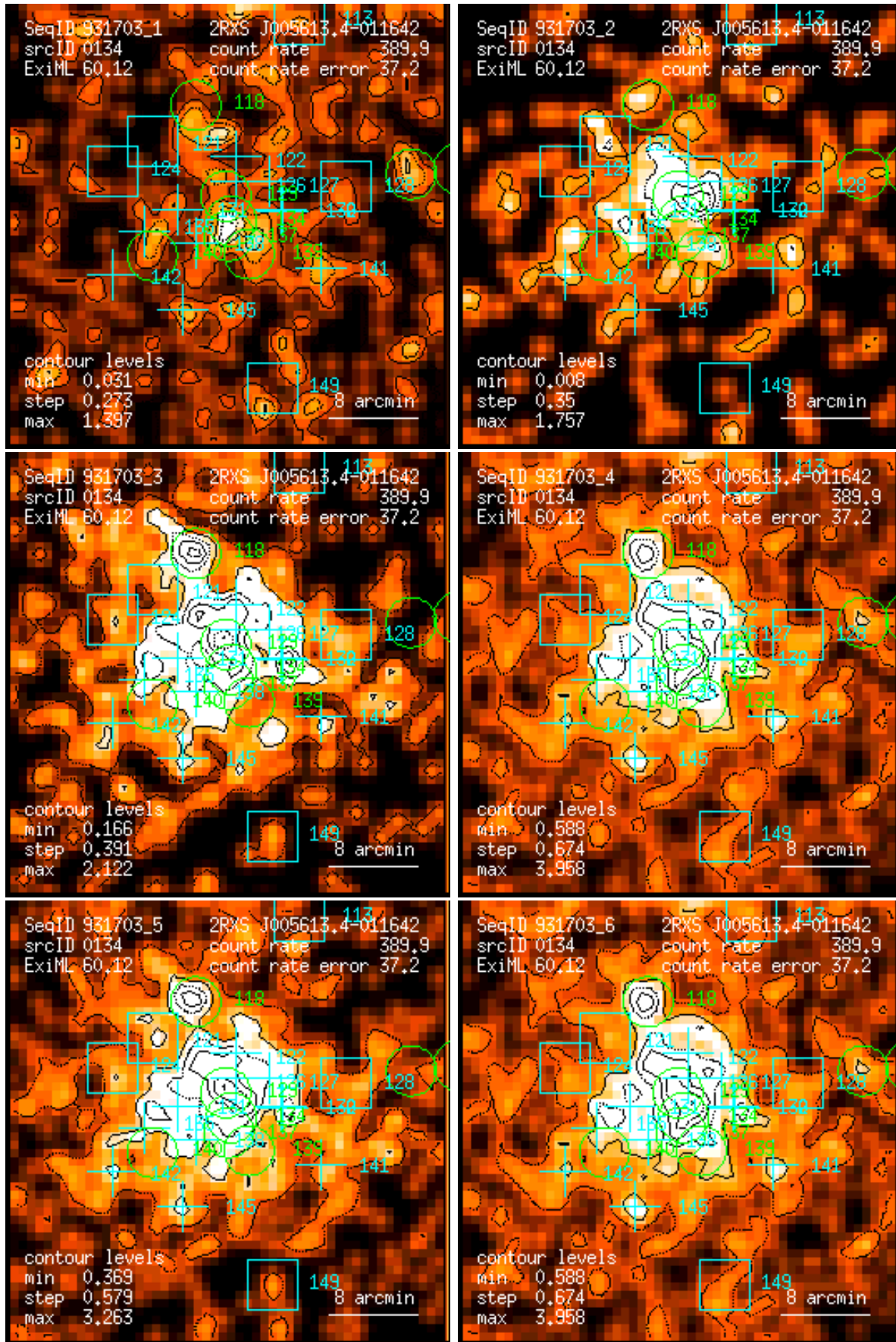
Figure 134: RASS 931703: detection 0134: band rate images, Gaussian filter: (1) PSPC channels 11 – 41, (2) 52 – 90, (3) 91 – 201, (4) 11 – 235, (5) 52 – 201, (6) 11 – 201. Broad band rates in counts/ks. Band rate contour levels in counts/ks/arcmin 2 .
