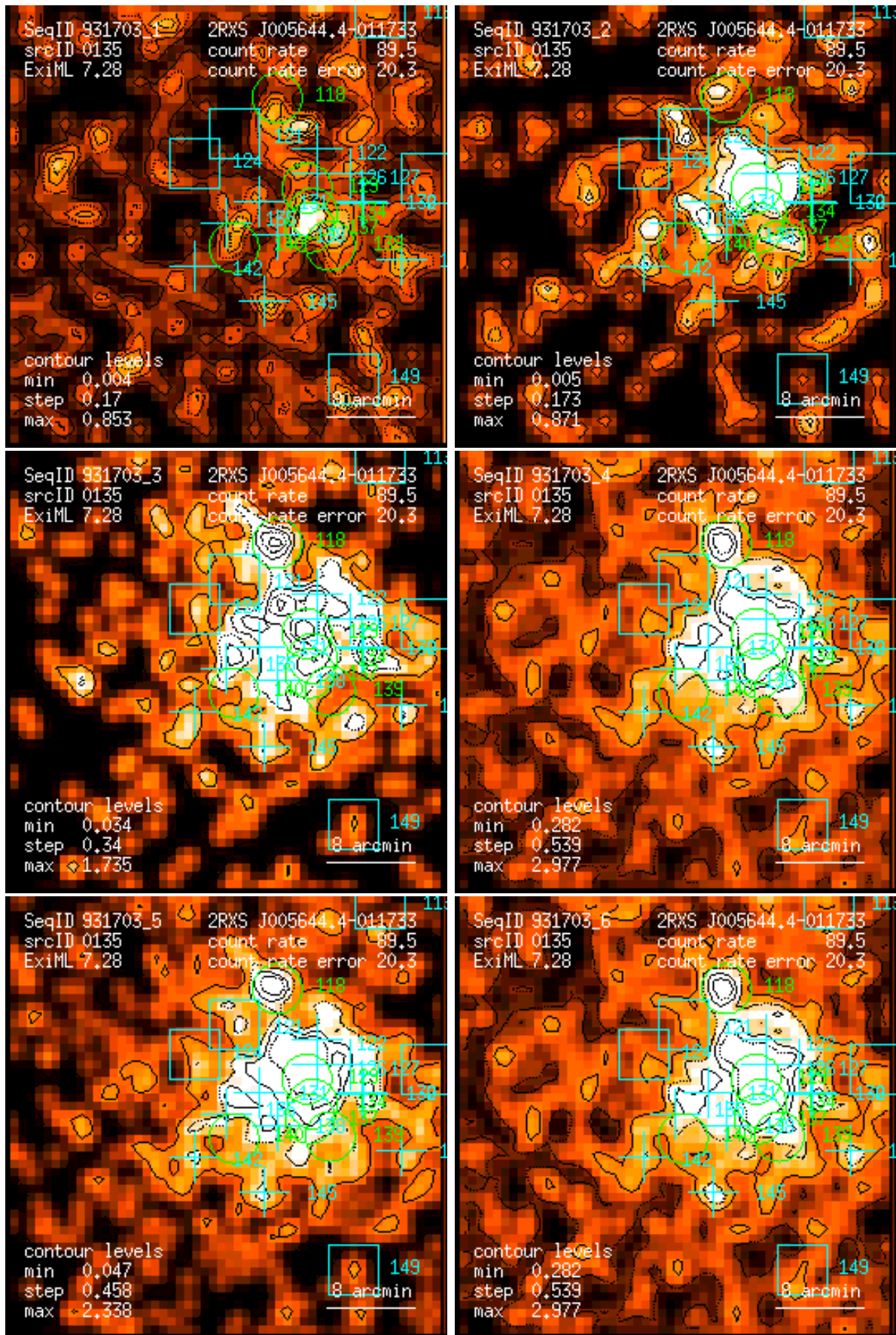
Figure 135: RASS 931703: detection 0135: band rate images, Gaussian filter: (1) PSPC channels 11 – 41, (2) 52 – 90, (3) 91 – 201, (4) 11 – 235, (5) 52 – 201, (6) 11 – 201. Broad band rates in counts/ks. Band rate contour levels in counts/ks/arcmin 2 .
