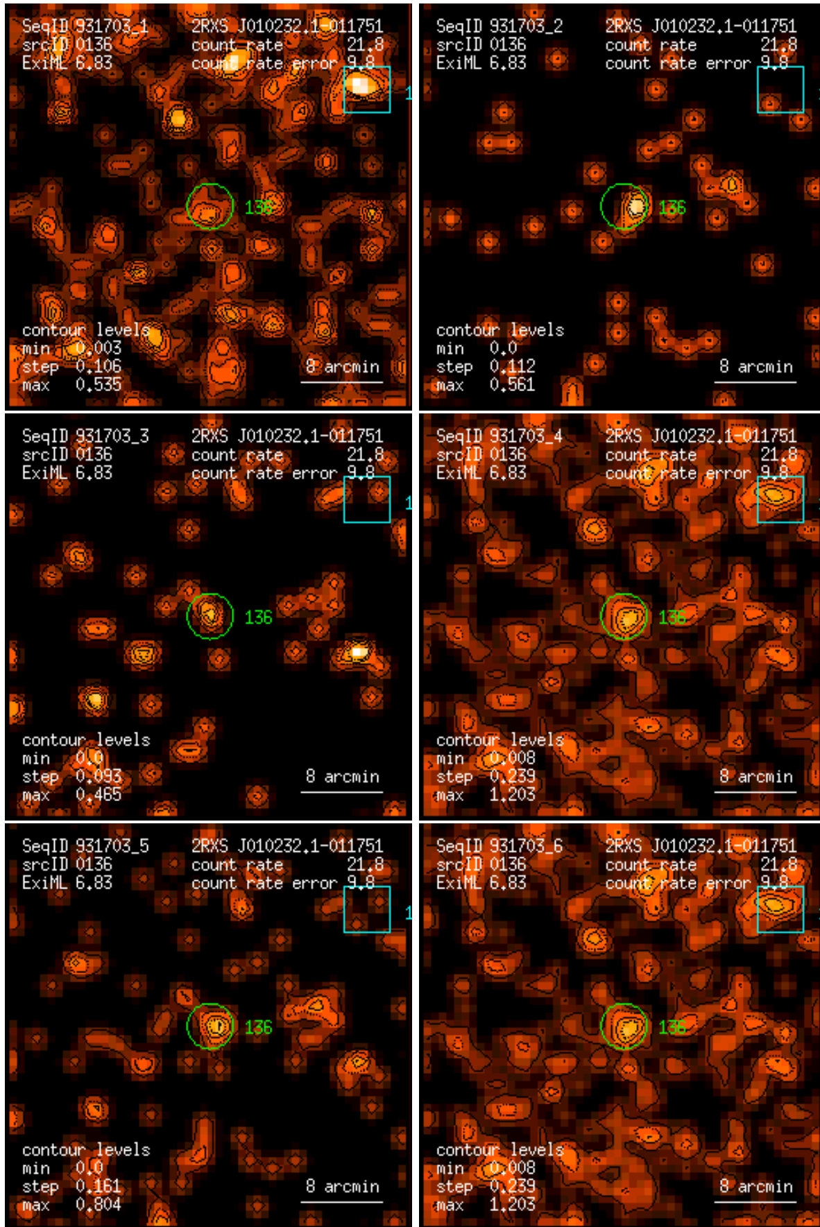
Figure 136: RASS 931703: detection 0136: band rate images, Gaussian filter: (1) PSPC channels 11 – 41, (2) 52 – 90, (3) 91 – 201, (4) 11 – 235, (5) 52 – 201, (6) 11 – 201. Broad band rates in counts/ks. Band rate contour levels in counts/ks/arcmin 2 .
