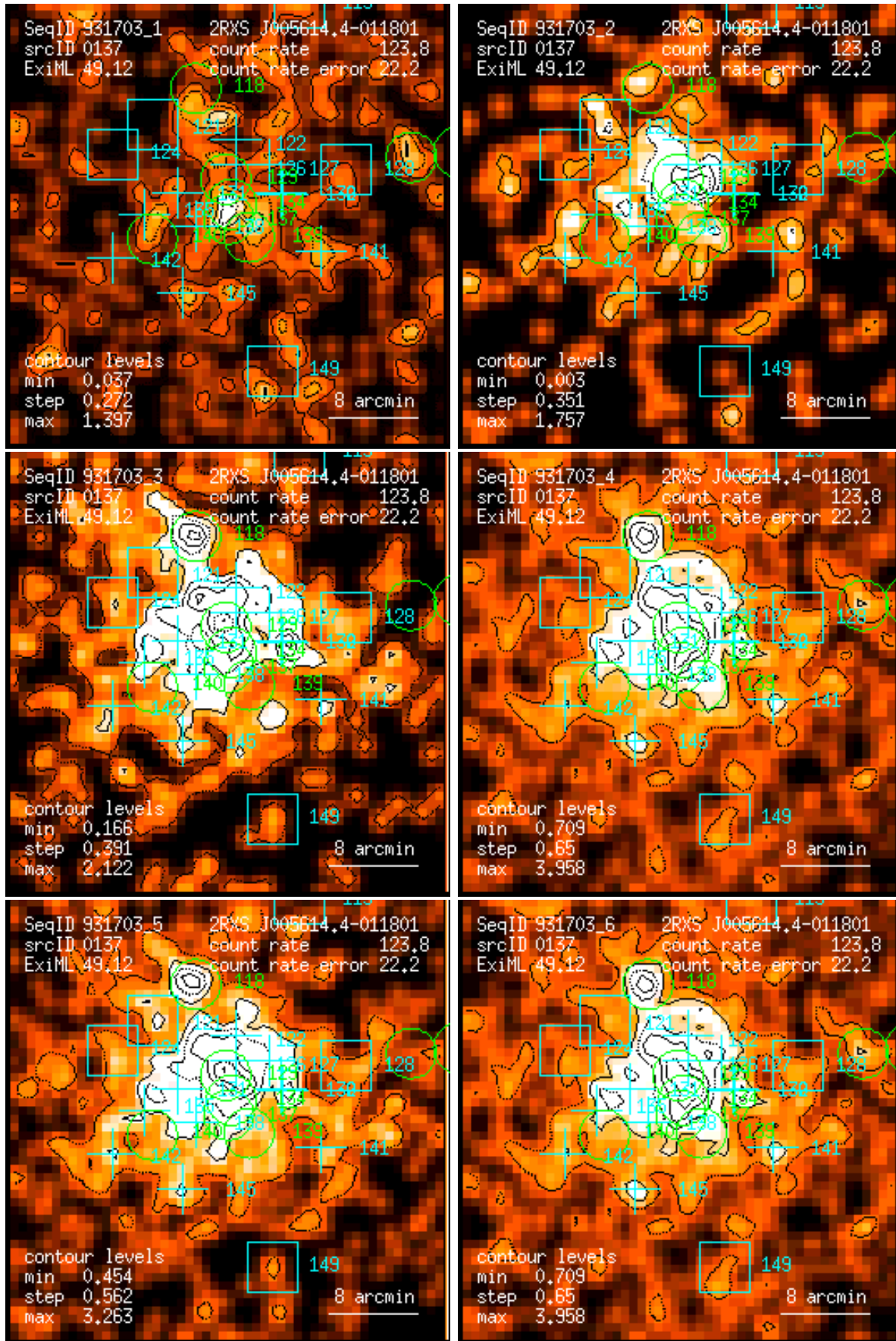
Figure 137: RASS 931703: detection 0137: band rate images, Gaussian filter: (1) PSPC channels 11 – 41, (2) 52 – 90, (3) 91 – 201, (4) 11 – 235, (5) 52 – 201, (6) 11 – 201. Broad band rates in counts/ks. Band rate contour levels in counts/ks/arcmin 2 .
