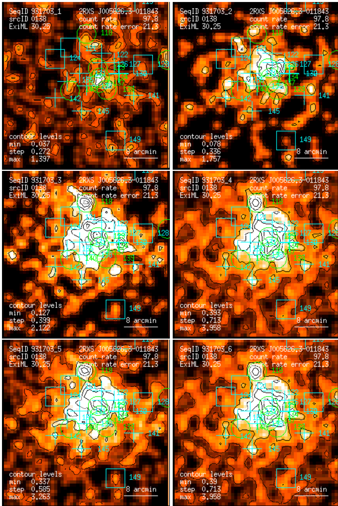
Figure 138: RASS 931703: detection 0138: band rate images, Gaussian filter: (1) PSPC channels 11 – 41, (2) 52 – 90, (3) 91 – 201, (4) 11 – 235, (5) 52 – 201, (6) 11 – 201. Broad band rates in counts/ks. Band rate contour levels in counts/ks/arcmin 2 .
