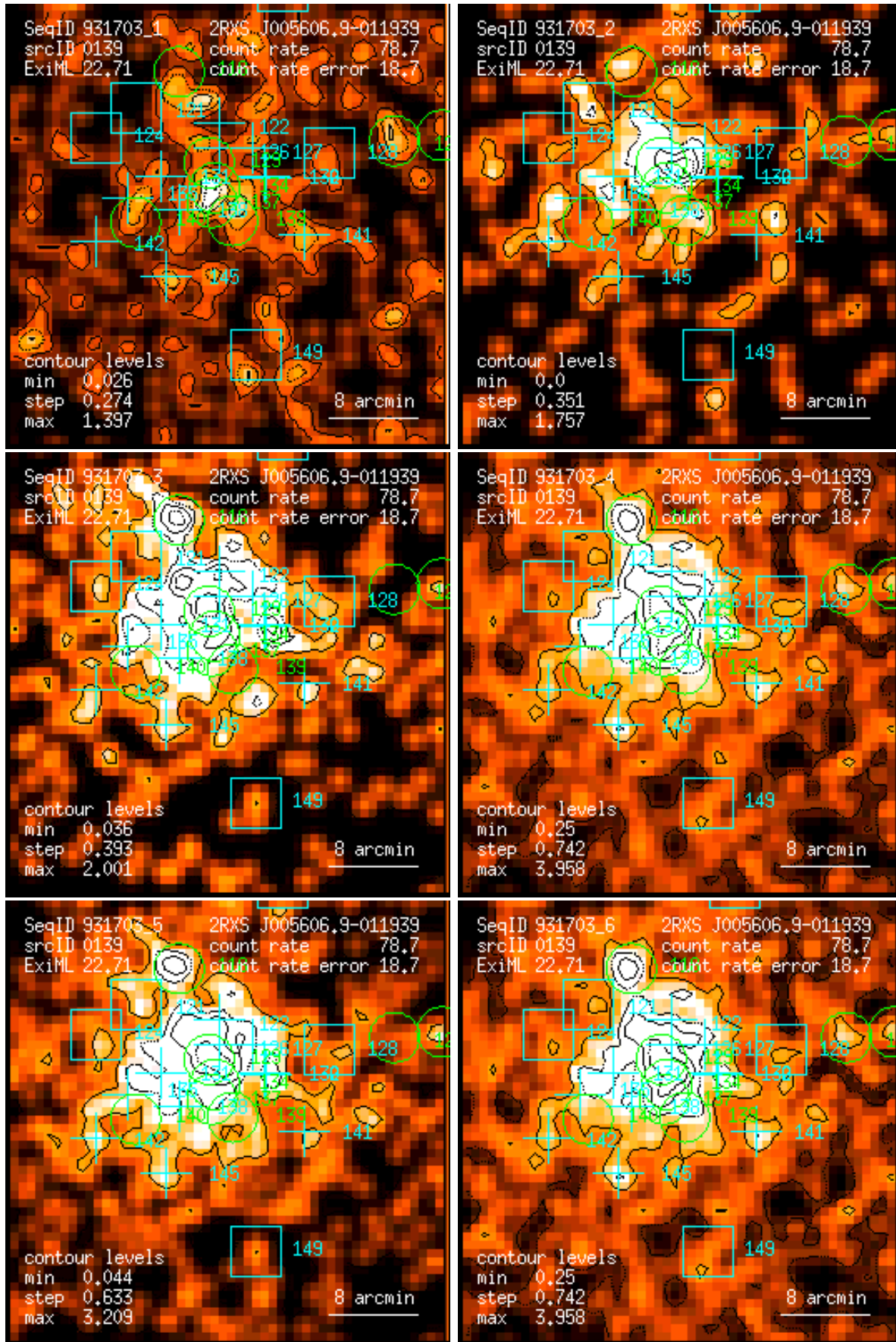
Figure 139: RASS 931703: detection 0139: band rate images, Gaussian filter: (1) PSPC channels 11 – 41, (2) 52 – 90, (3) 91 – 201, (4) 11 – 235, (5) 52 – 201, (6) 11 – 201. Broad band rates in counts/ks. Band rate contour levels in counts/ks/arcmin 2 .
