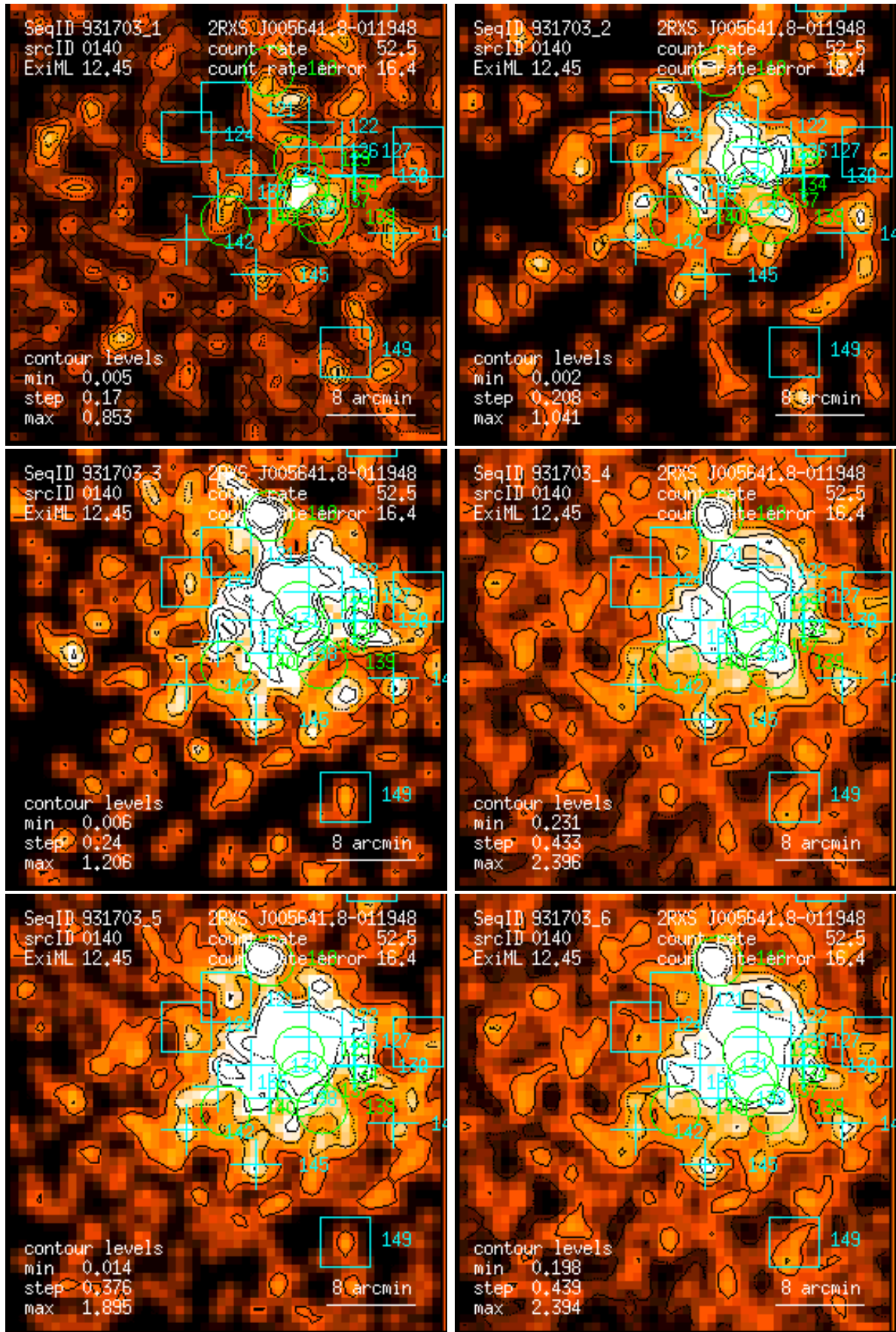
Figure 140: RASS 931703: detection 0140: band rate images, Gaussian filter: (1) PSPC channels 11 – 41, (2) 52 – 90, (3) 91 – 201, (4) 11 – 235, (5) 52 – 201, (6) 11 – 201. Broad band rates in counts/ks. Band rate contour levels in counts/ks/arcmin 2 .
