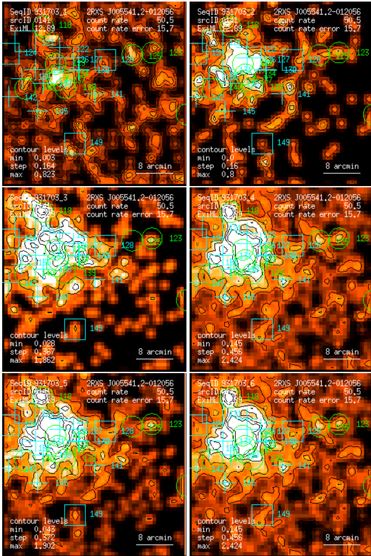
Figure 141: RASS 931703: detection 0141: band rate images, Gaussian filter: (1) PSPC channels 11 – 41, (2) 52 – 90, (3) 91 – 201, (4) 11 – 235, (5) 52 – 201, (6) 11 – 201. Broad band rates in counts/ks. Band rate contour levels in counts/ks/arcmin 2 .
