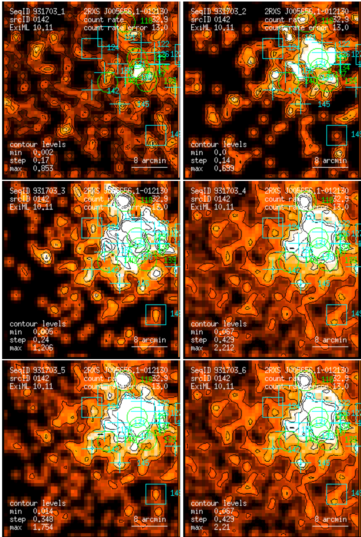
Figure 142: RASS 931703: detection 0142: band rate images, Gaussian filter: (1) PSPC channels 11 – 41, (2) 52 – 90, (3) 91 – 201, (4) 11 – 235, (5) 52 – 201, (6) 11 – 201. Broad band rates in counts/ks. Band rate contour levels in counts/ks/arcmin 2 .
