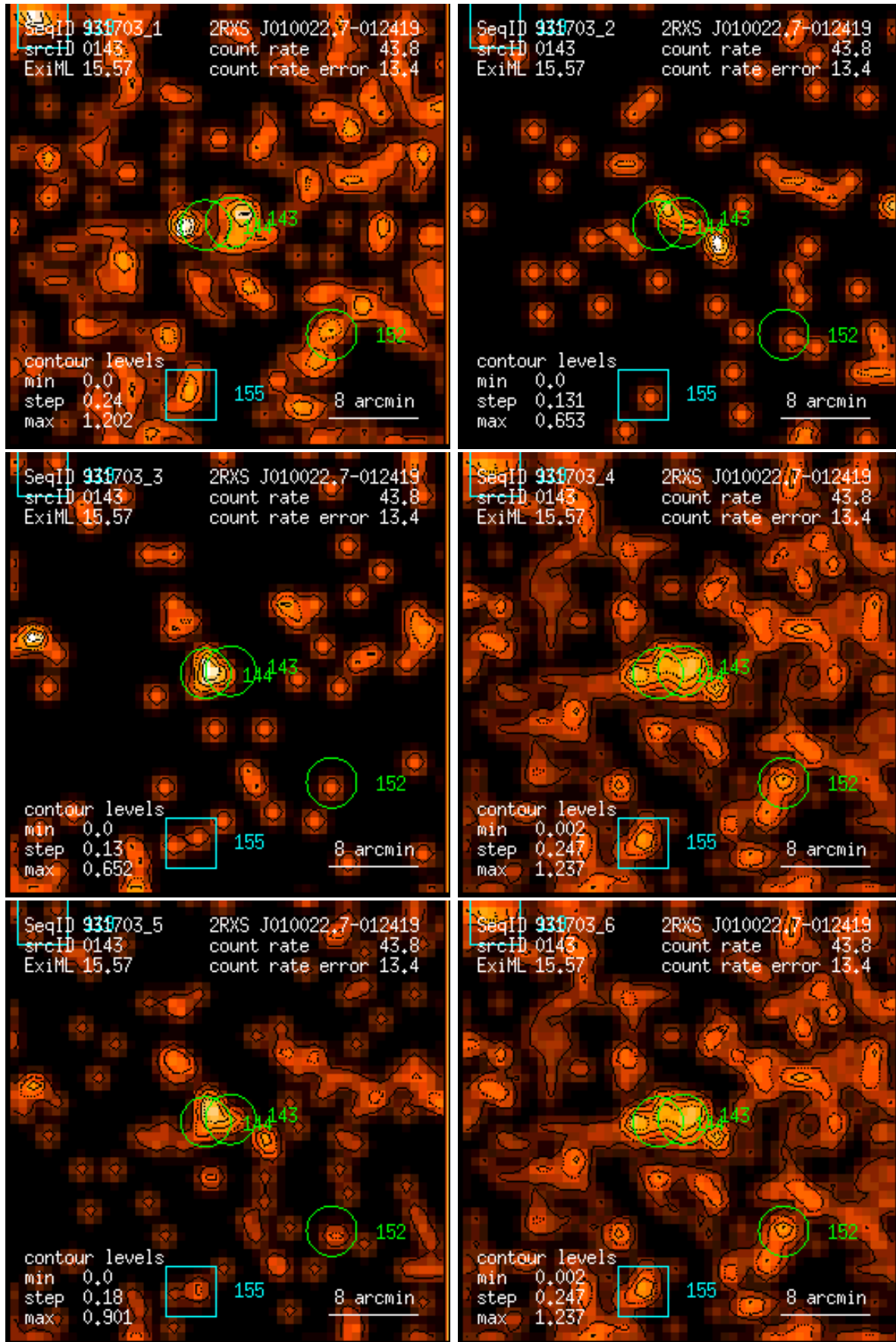
Figure 143: RASS 931703: detection 0143: band rate images, Gaussian filter: (1) PSPC channels 11 – 41, (2) 52 – 90, (3) 91 – 201, (4) 11 – 235, (5) 52 – 201, (6) 11 – 201. Broad band rates in counts/ks. Band rate contour levels in counts/ks/arcmin 2 .
