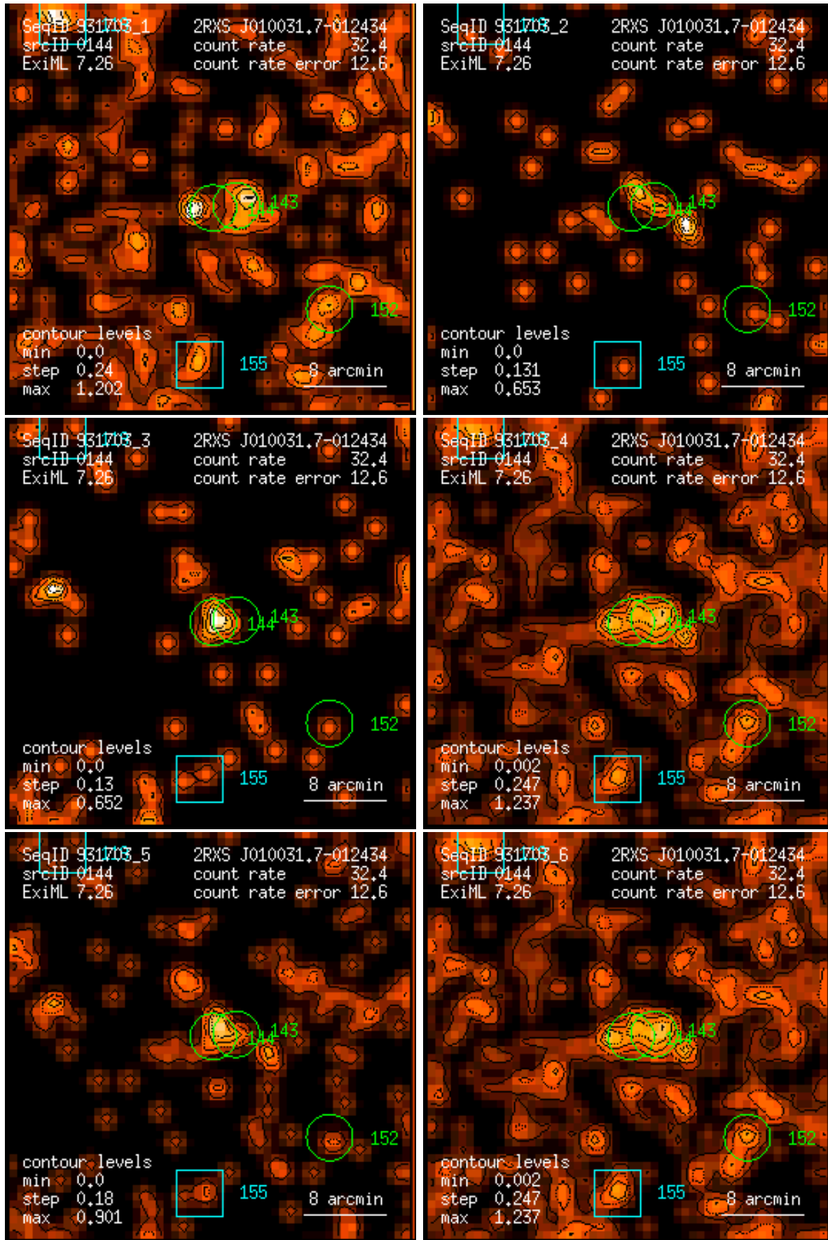
Figure 144: RASS 931703: detection 0144: band rate images, Gaussian filter: (1) PSPC channels 11 – 41, (2) 52 – 90, (3) 91 – 201, (4) 11 – 235, (5) 52 – 201, (6) 11 – 201. Broad band rates in counts/ks. Band rate contour levels in counts/ks/arcmin 2 .
