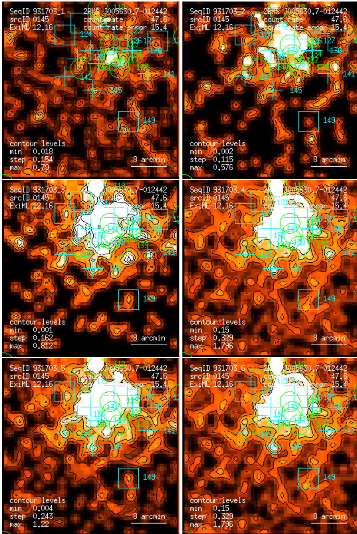
Figure 145: RASS 931703: detection 0145: band rate images, Gaussian filter: (1) PSPC channels 11 – 41, (2) 52 – 90, (3) 91 – 201, (4) 11 – 235, (5) 52 – 201, (6) 11 – 201. Broad band rates in counts/ks. Band rate contour levels in counts/ks/arcmin 2 .
