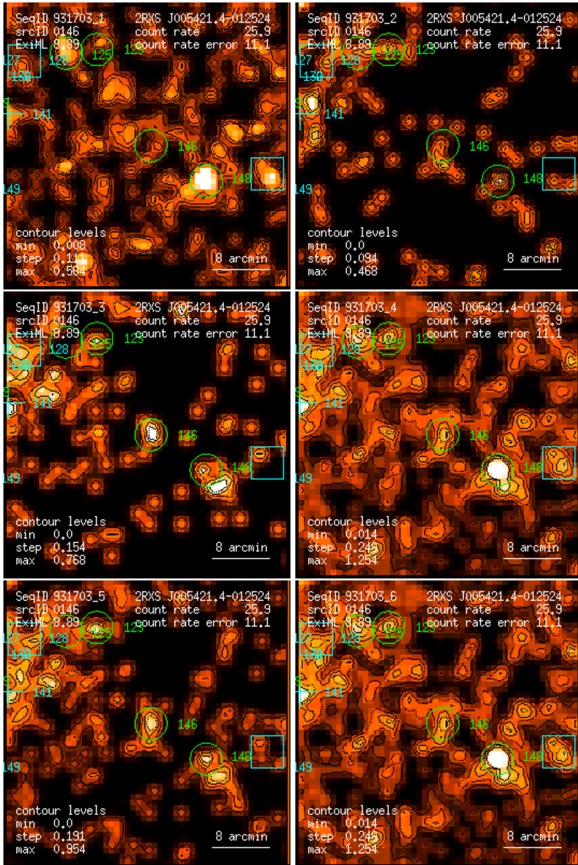
Figure 146: RASS 931703: detection 0146: band rate images, Gaussian filter: (1) PSPC channels 11 – 41, (2) 52 – 90, (3) 91 – 201, (4) 11 – 235, (5) 52 – 201, (6) 11 – 201. Broad band rates in counts/ks. Band rate contour levels in counts/ks/arcmin 2 .
