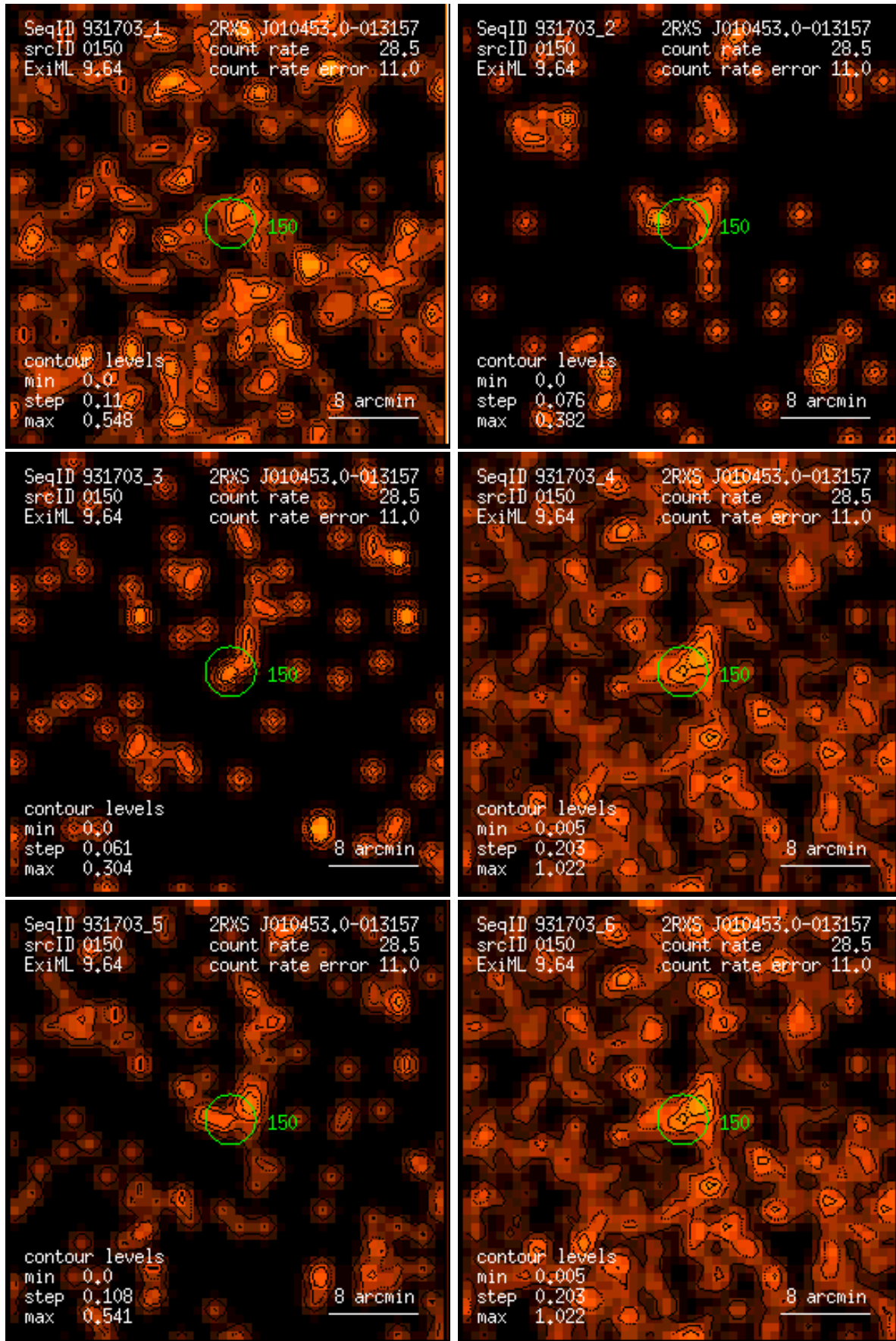
Figure 150: RASS 931703: detection 0150: band rate images, Gaussian filter: (1) PSPC channels 11 – 41, (2) 52 – 90, (3) 91 – 201, (4) 11 – 235, (5) 52 – 201, (6) 11 – 201. Broad band rates in counts/ks. Band rate contour levels in counts/ks/arcmin 2 .
