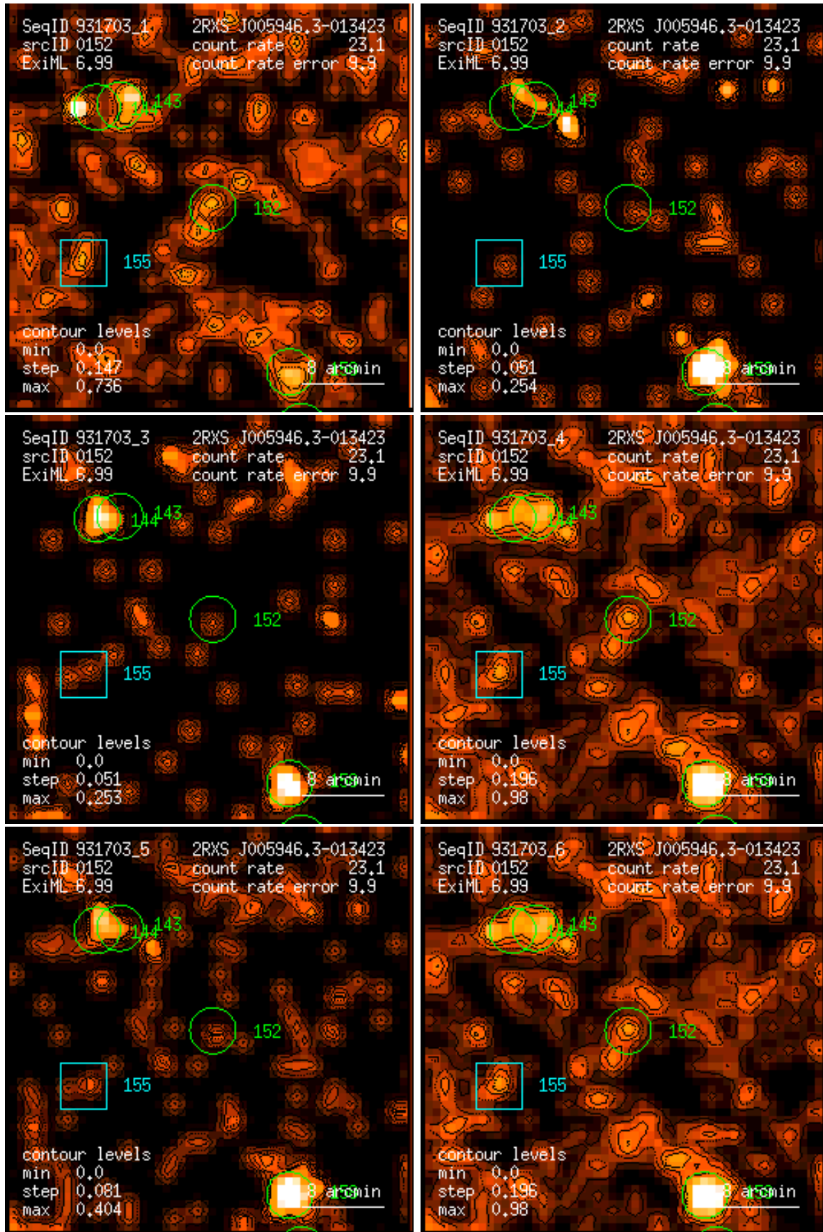
Figure 152: RASS 931703: detection 0152: band rate images, Gaussian filter: (1) PSPC channels 11 – 41, (2) 52 – 90, (3) 91 – 201, (4) 11 – 235, (5) 52 – 201, (6) 11 – 201. Broad band rates in counts/ks. Band rate contour levels in counts/ks/arcmin 2 .
