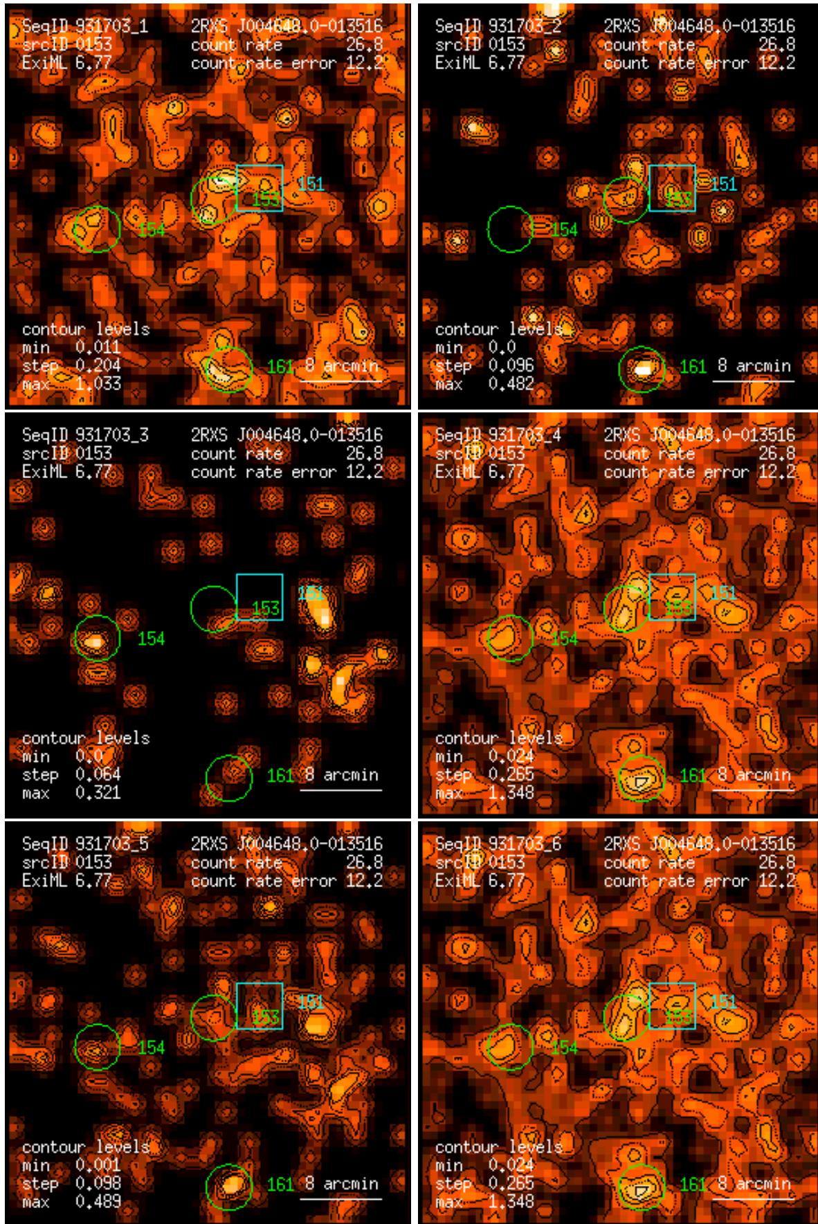
Figure 153: RASS 931703: detection 0153: band rate images, Gaussian filter: (1) PSPC channels 11 – 41, (2) 52 – 90, (3) 91 – 201, (4) 11 – 235, (5) 52 – 201, (6) 11 – 201. Broad band rates in counts/ks. Band rate contour levels in counts/ks/arcmin 2 .
