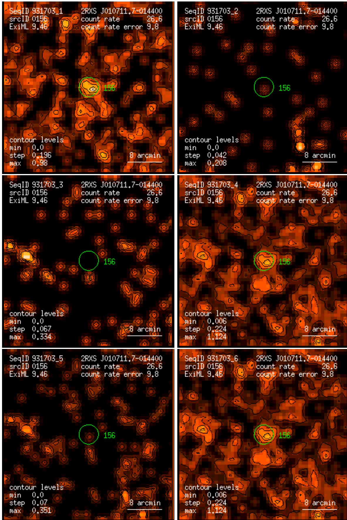
Figure 156: RASS 931703: detection 0156: band rate images, Gaussian filter: (1) PSPC channels 11 – 41, (2) 52 – 90, (3) 91 – 201, (4) 11 – 235, (5) 52 – 201, (6) 11 – 201. Broad band rates in counts/ks. Band rate contour levels in counts/ks/arcmin 2 .
