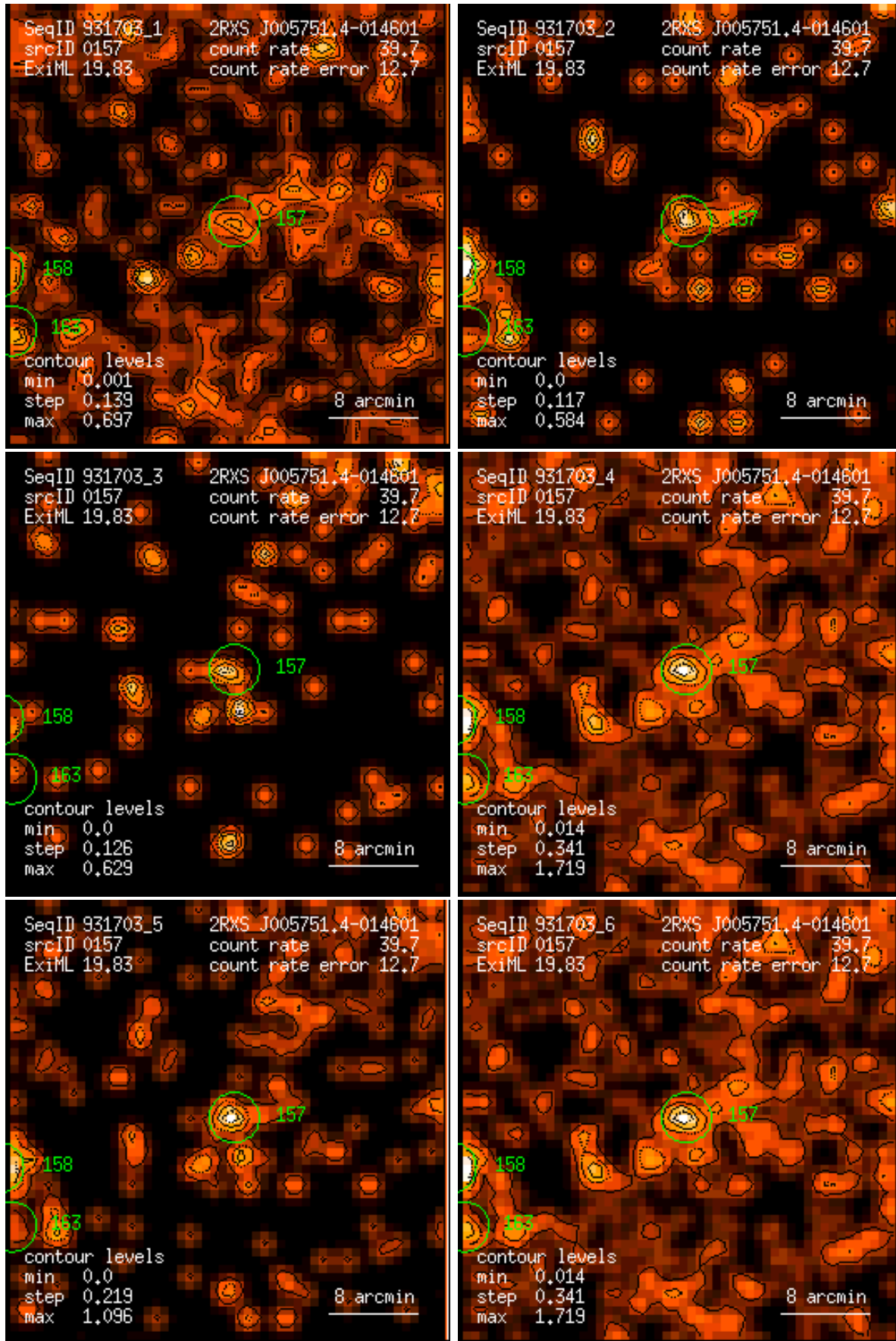
Figure 157: RASS 931703: detection 0157: band rate images, Gaussian filter: (1) PSPC channels 11 – 41, (2) 52 – 90, (3) 91 – 201, (4) 11 – 235, (5) 52 – 201, (6) 11 – 201. Broad band rates in counts/ks. Band rate contour levels in counts/ks/arcmin 2 .
