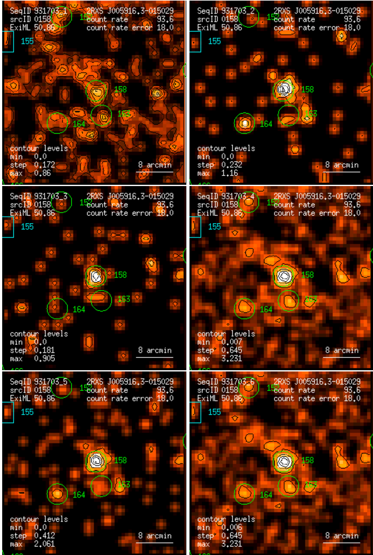
Figure 158: RASS 931703: detection 0158: band rate images, Gaussian filter: (1) PSPC channels 11 – 41, (2) 52 – 90, (3) 91 – 201, (4) 11 – 235, (5) 52 – 201, (6) 11 – 201. Broad band rates in counts/ks. Band rate contour levels in counts/ks/arcmin 2 .
