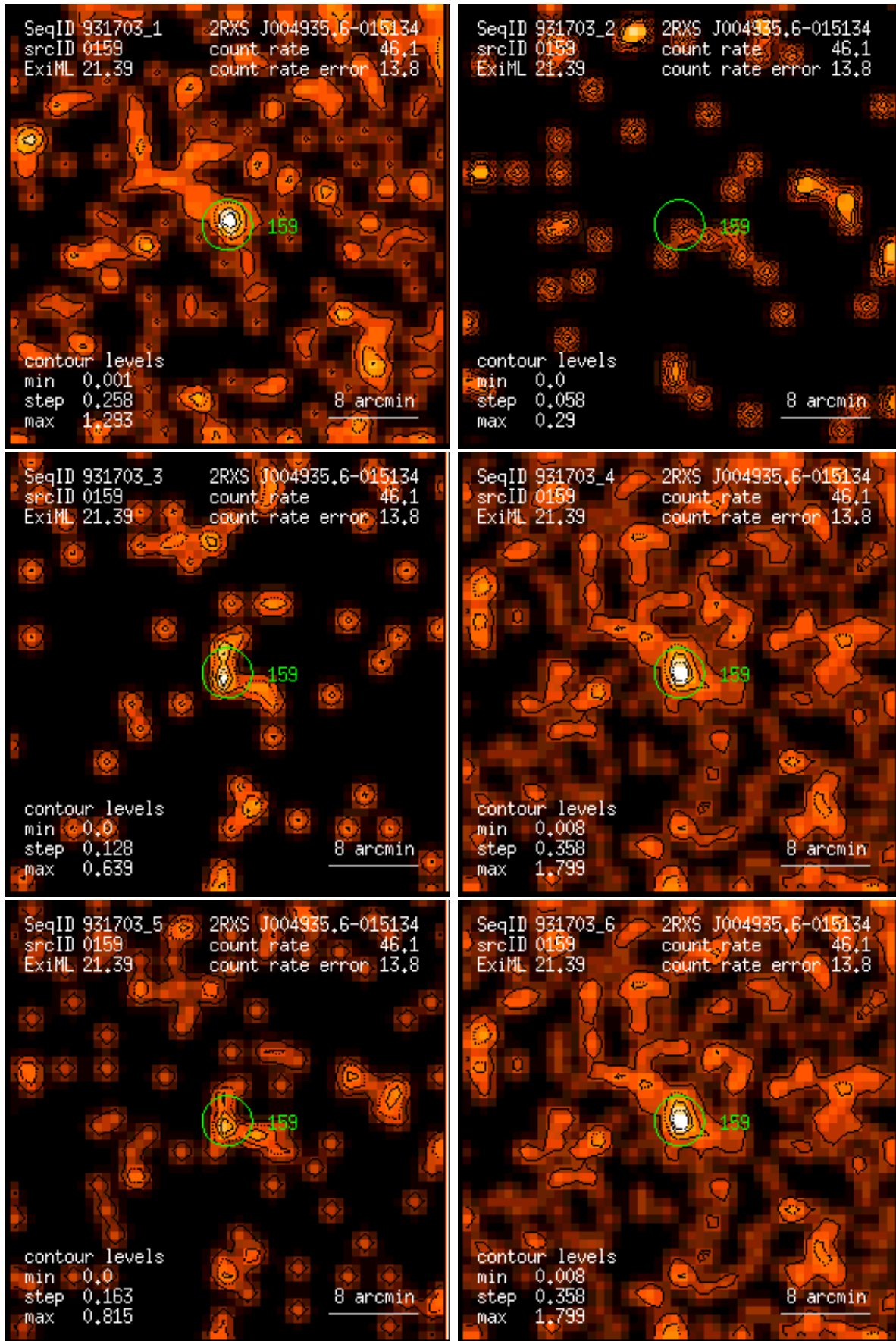
Figure 159: RASS 931703: detection 0159: band rate images, Gaussian filter: (1) PSPC channels 11 – 41, (2) 52 – 90, (3) 91 – 201, (4) 11 – 235, (5) 52 – 201, (6) 11 – 201. Broad band rates in counts/ks. Band rate contour levels in counts/ks/arcmin 2 .
