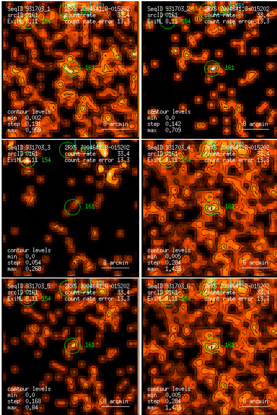
Figure 161: RASS 931703: detection 0161: band rate images, Gaussian filter: (1) PSPC channels 11 – 41, (2) 52 – 90, (3) 91 – 201, (4) 11 – 235, (5) 52 – 201, (6) 11 – 201. Broad band rates in counts/ks. Band rate contour levels in counts/ks/arcmin 2 .
