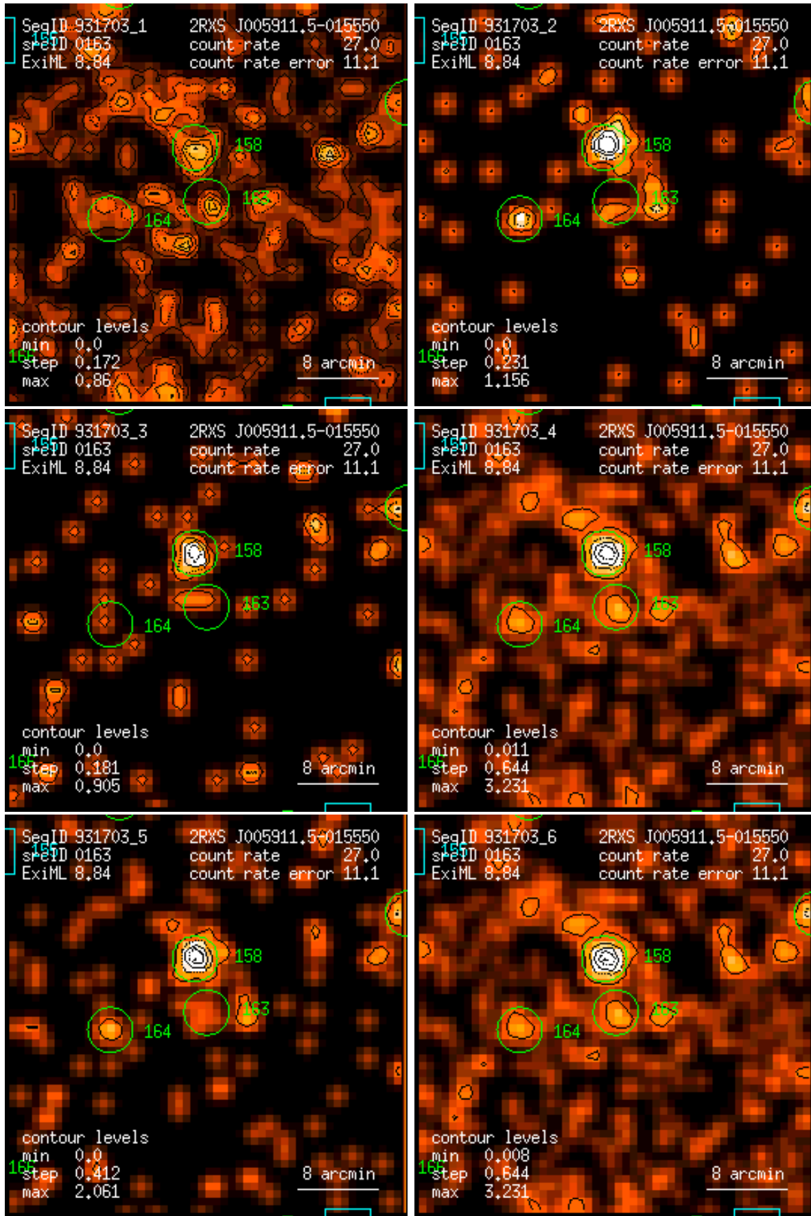
Figure 163: RASS 931703: detection 0163: band rate images, Gaussian filter: (1) PSPC channels 11 – 41, (2) 52 – 90, (3) 91 – 201, (4) 11 – 235, (5) 52 – 201, (6) 11 – 201. Broad band rates in counts/ks. Band rate contour levels in counts/ks/arcmin 2 .
