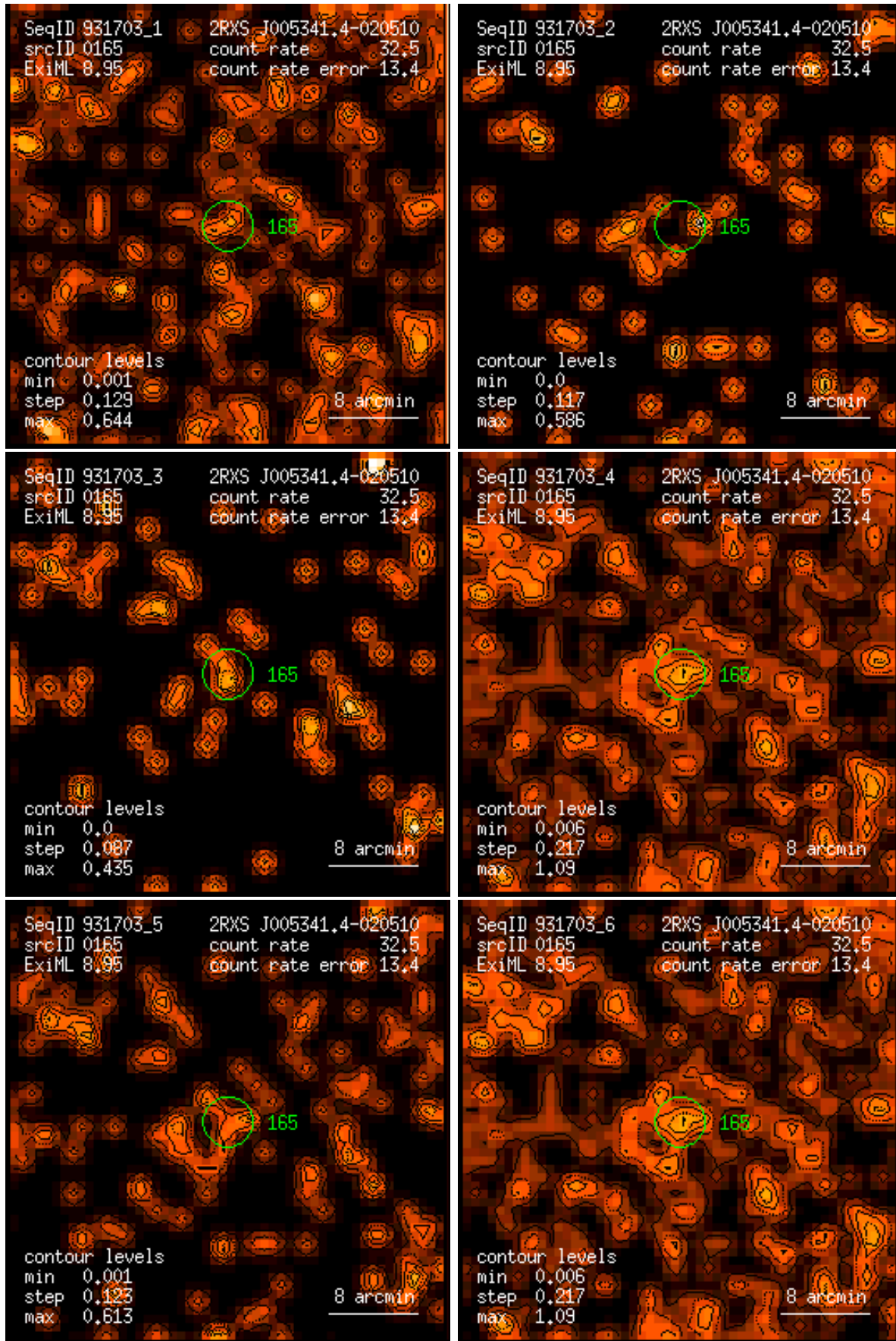
Figure 165: RASS 931703: detection 0165: band rate images, Gaussian filter: (1) PSPC channels 11 – 41, (2) 52 – 90, (3) 91 – 201, (4) 11 – 235, (5) 52 – 201, (6) 11 – 201. Broad band rates in counts/ks. Band rate contour levels in counts/ks/arcmin 2 .
