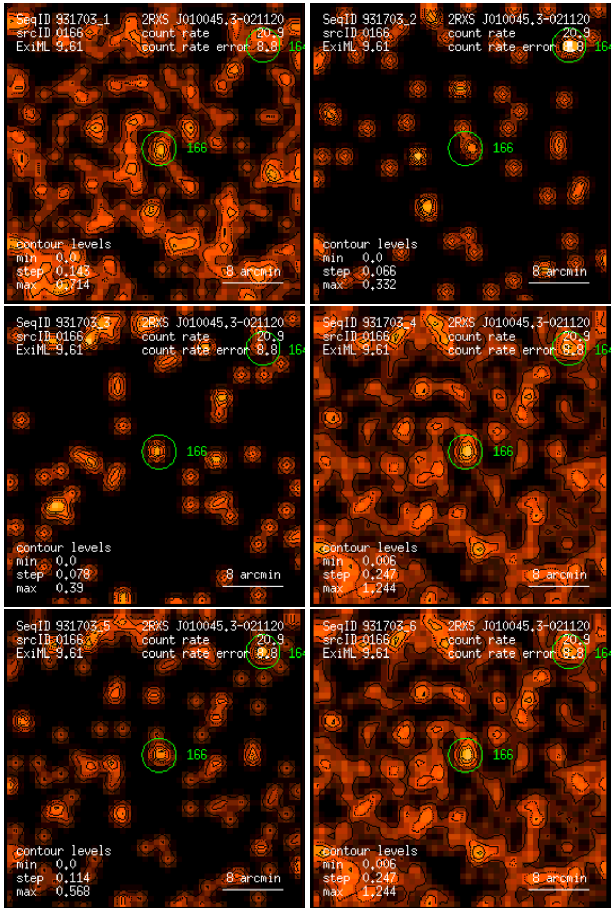
Figure 166: RASS 931703: detection 0166: band rate images, Gaussian filter: (1) PSPC channels 11 – 41, (2) 52 – 90, (3) 91 – 201, (4) 11 – 235, (5) 52 – 201, (6) 11 – 201. Broad band rates in counts/ks. Band rate contour levels in counts/ks/arcmin 2 .
