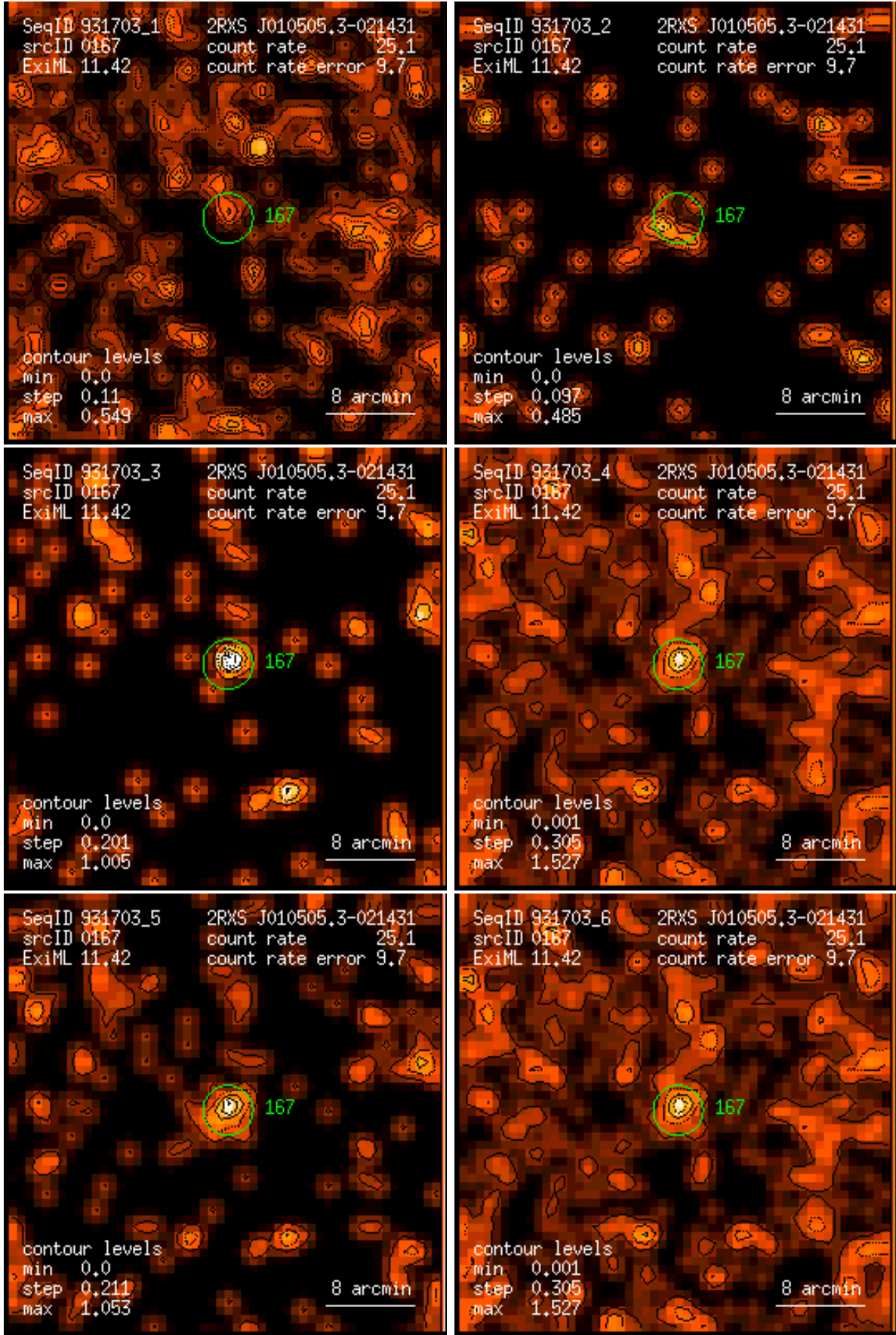
Figure 167: RASS 931703: detection 0167: band rate images, Gaussian filter: (1) PSPC channels 11 – 41, (2) 52 – 90, (3) 91 – 201, (4) 11 – 235, (5) 52 – 201, (6) 11 – 201. Broad band rates in counts/ks. Band rate contour levels in counts/ks/arcmin 2 .
