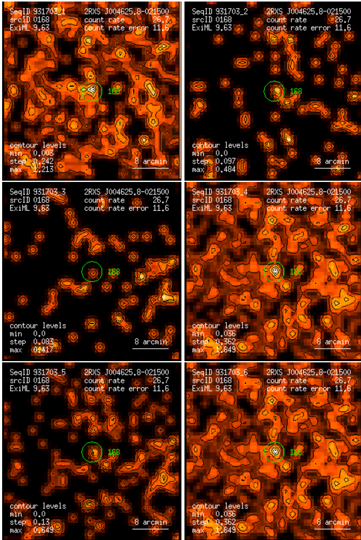
Figure 168: RASS 931703: detection 0168: band rate images, Gaussian filter: (1) PSPC channels 11 – 41, (2) 52 – 90, (3) 91 – 201, (4) 11 – 235, (5) 52 – 201, (6) 11 – 201. Broad band rates in counts/ks. Band rate contour levels in counts/ks/arcmin 2 .
