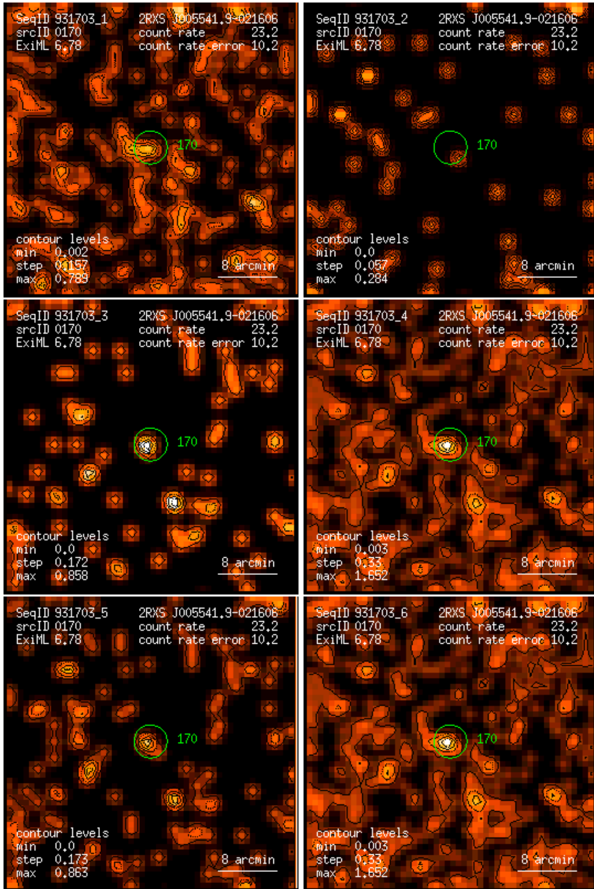
Figure 170: RASS 931703: detection 0170: band rate images, Gaussian filter: (1) PSPC channels 11 – 41, (2) 52 – 90, (3) 91 – 201, (4) 11 – 235, (5) 52 – 201, (6) 11 – 201. Broad band rates in counts/ks. Band rate contour levels in counts/ks/arcmin 2 .
