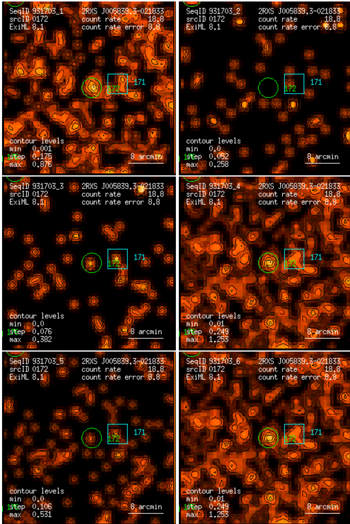
Figure 172: RASS 931703: detection 0172: band rate images, Gaussian filter: (1) PSPC channels 11 – 41, (2) 52 – 90, (3) 91 – 201, (4) 11 – 235, (5) 52 – 201, (6) 11 – 201. Broad band rates in counts/ks. Band rate contour levels in counts/ks/arcmin 2 .
