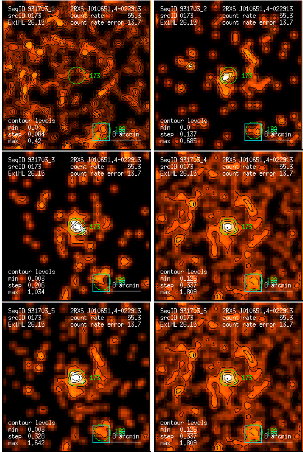
Figure 173: RASS 931703: detection 0173: band rate images, Gaussian filter: (1) PSPC channels 11 – 41, (2) 52 – 90, (3) 91 – 201, (4) 11 – 235, (5) 52 – 201, (6) 11 – 201. Broad band rates in counts/ks. Band rate contour levels in counts/ks/arcmin 2 .
