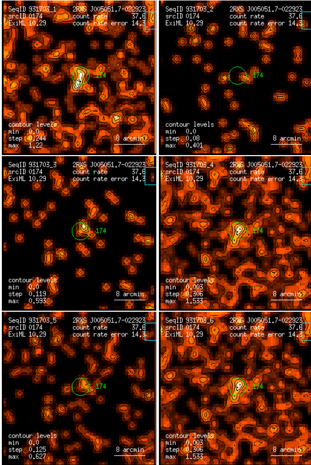
Figure 174: RASS 931703: detection 0174: band rate images, Gaussian filter: (1) PSPC channels 11 – 41, (2) 52 – 90, (3) 91 – 201, (4) 11 – 235, (5) 52 – 201, (6) 11 – 201. Broad band rates in counts/ks. Band rate contour levels in counts/ks/arcmin 2 .
