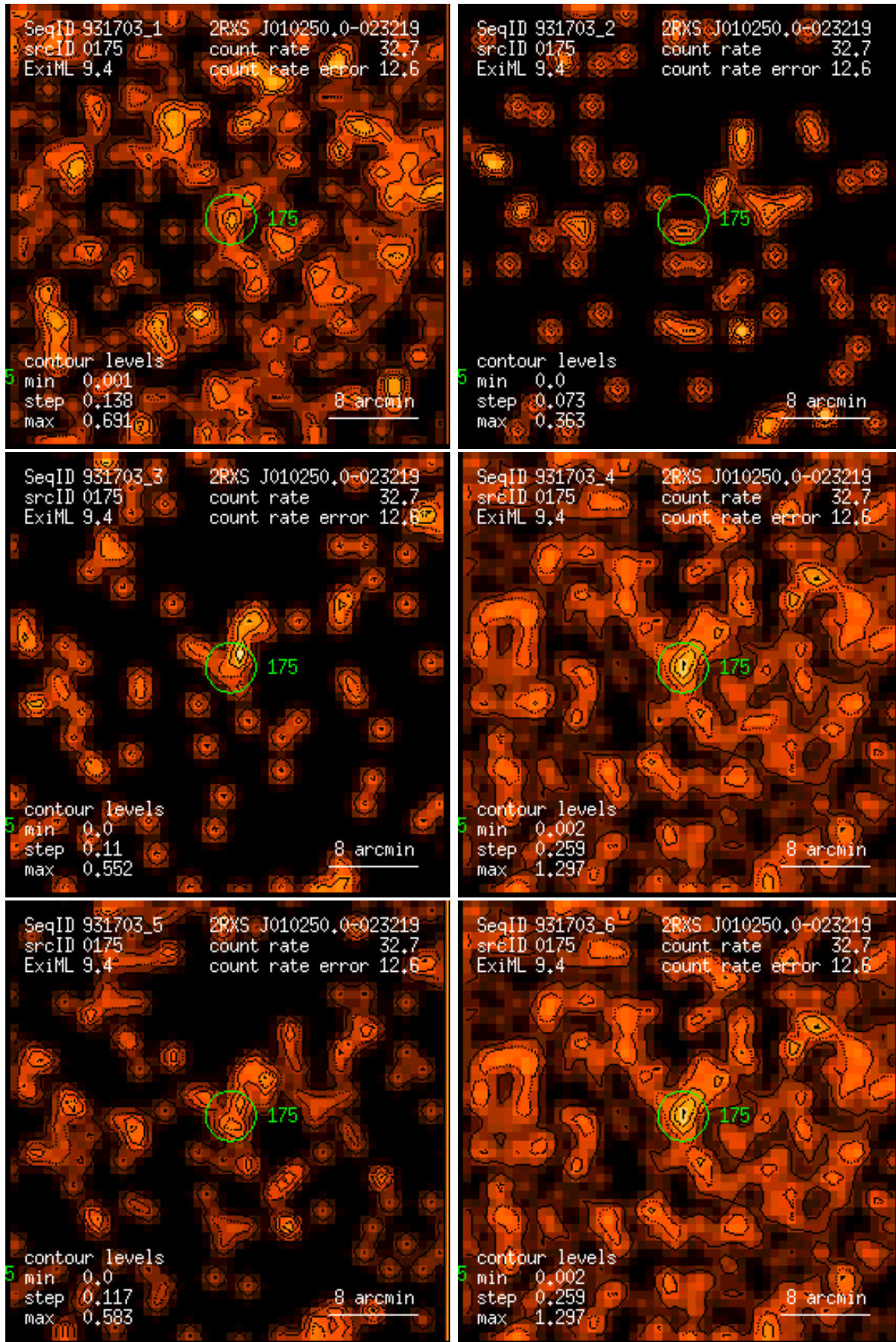
Figure 175: RASS 931703: detection 0175: band rate images, Gaussian filter: (1) PSPC channels 11 – 41, (2) 52 – 90, (3) 91 – 201, (4) 11 – 235, (5) 52 – 201, (6) 11 – 201. Broad band rates in counts/ks. Band rate contour levels in counts/ks/arcmin 2 .
