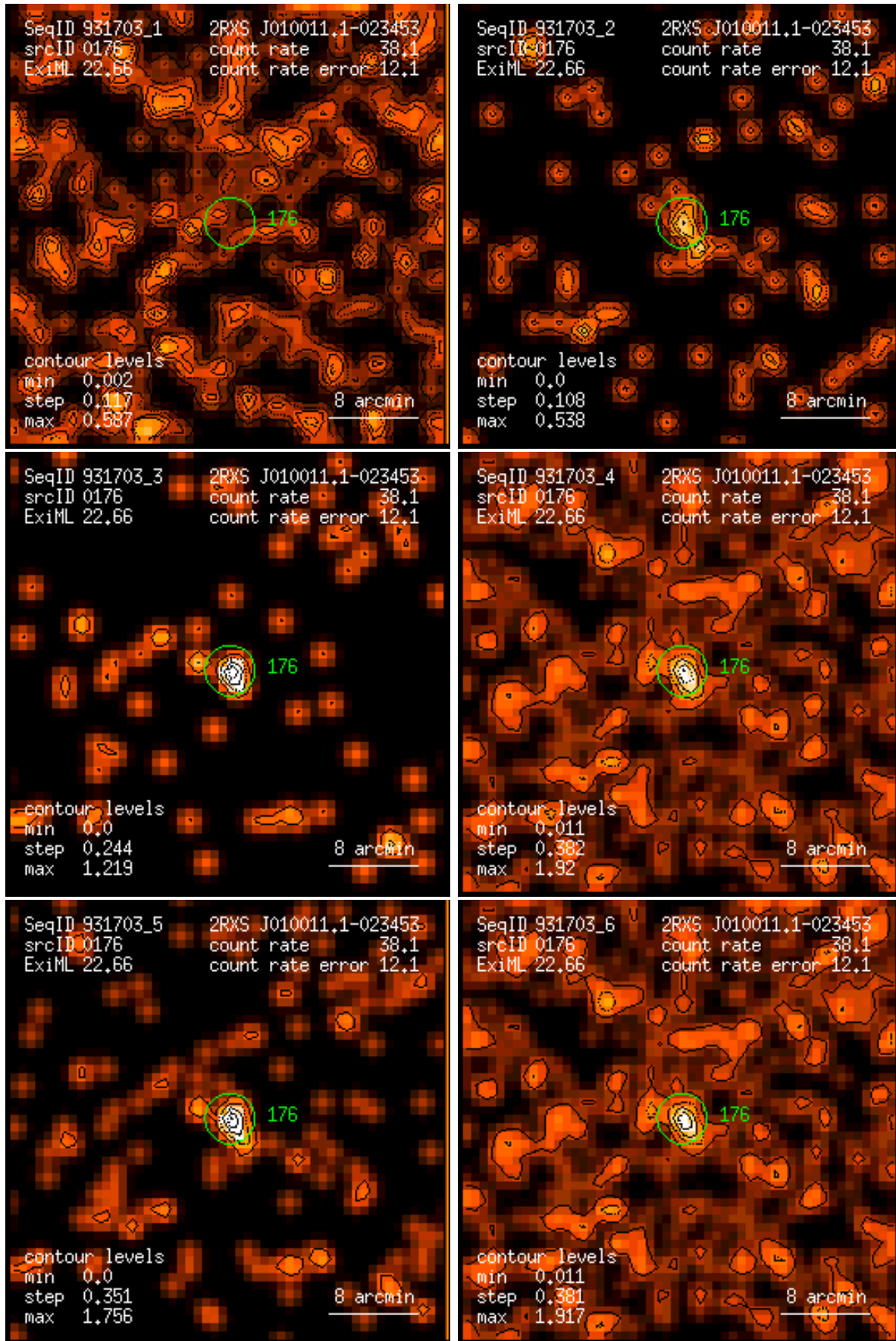
Figure 176: RASS 931703: detection 0176: band rate images, Gaussian filter: (1) PSPC channels 11 – 41, (2) 52 – 90, (3) 91 – 201, (4) 11 – 235, (5) 52 – 201, (6) 11 – 201. Broad band rates in counts/ks. Band rate contour levels in counts/ks/arcmin 2 .
