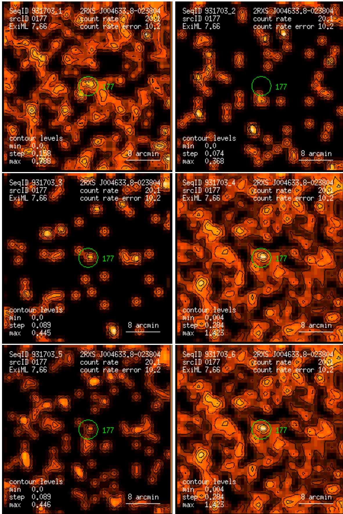
Figure 177: RASS 931703: detection 0177: band rate images, Gaussian filter: (1) PSPC channels 11 – 41, (2) 52 – 90, (3) 91 – 201, (4) 11 – 235, (5) 52 – 201, (6) 11 – 201. Broad band rates in counts/ks. Band rate contour levels in counts/ks/arcmin 2 .
