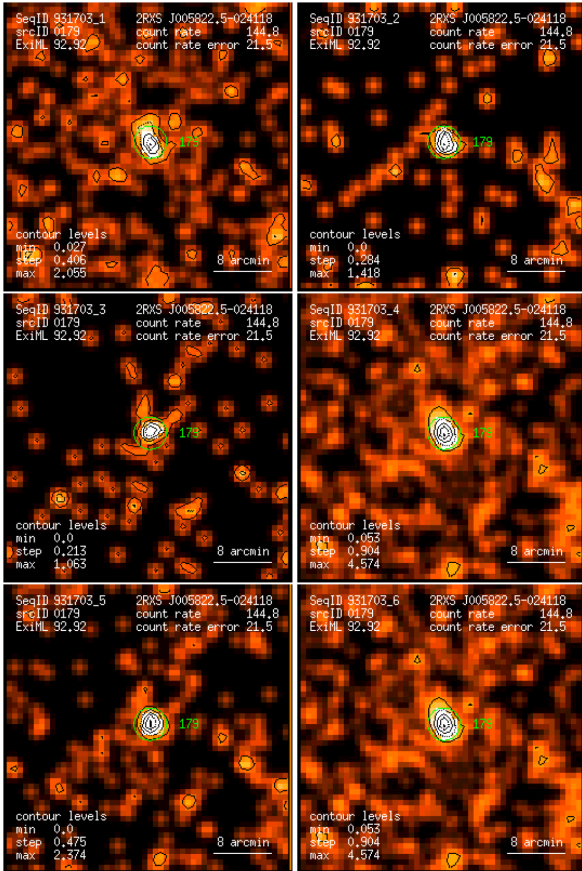
Figure 179: RASS 931703: detection 0179: band rate images, Gaussian filter: (1) PSPC channels 11 – 41, (2) 52 – 90, (3) 91 – 201, (4) 11 – 235, (5) 52 – 201, (6) 11 – 201. Broad band rates in counts/ks. Band rate contour levels in counts/ks/arcmin 2 .
