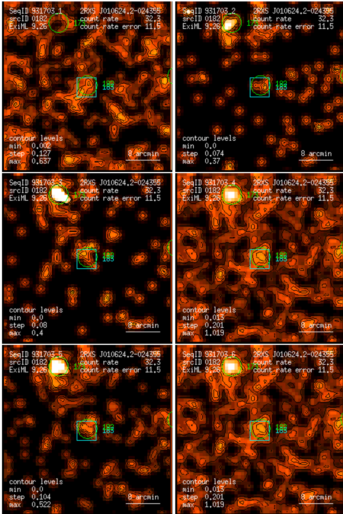
Figure 182: RASS 931703: detection 0182: band rate images, Gaussian filter: (1) PSPC channels 11 – 41, (2) 52 – 90, (3) 91 – 201, (4) 11 – 235, (5) 52 – 201, (6) 11 – 201. Broad band rates in counts/ks. Band rate contour levels in counts/ks/arcmin 2 .
