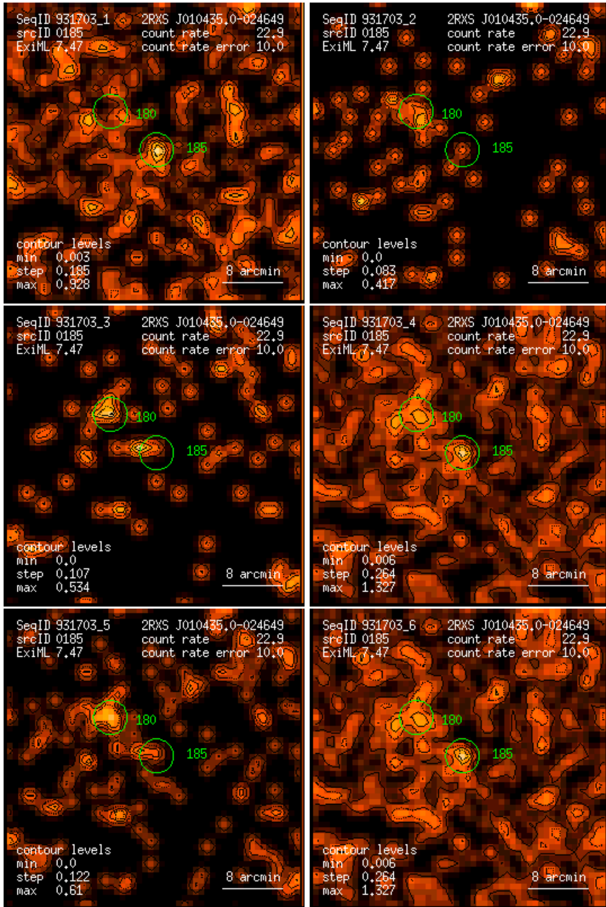
Figure 185: RASS 931703: detection 0185: band rate images, Gaussian filter: (1) PSPC channels 11 – 41, (2) 52 – 90, (3) 91 – 201, (4) 11 – 235, (5) 52 – 201, (6) 11 – 201. Broad band rates in counts/ks. Band rate contour levels in counts/ks/arcmin 2 .
