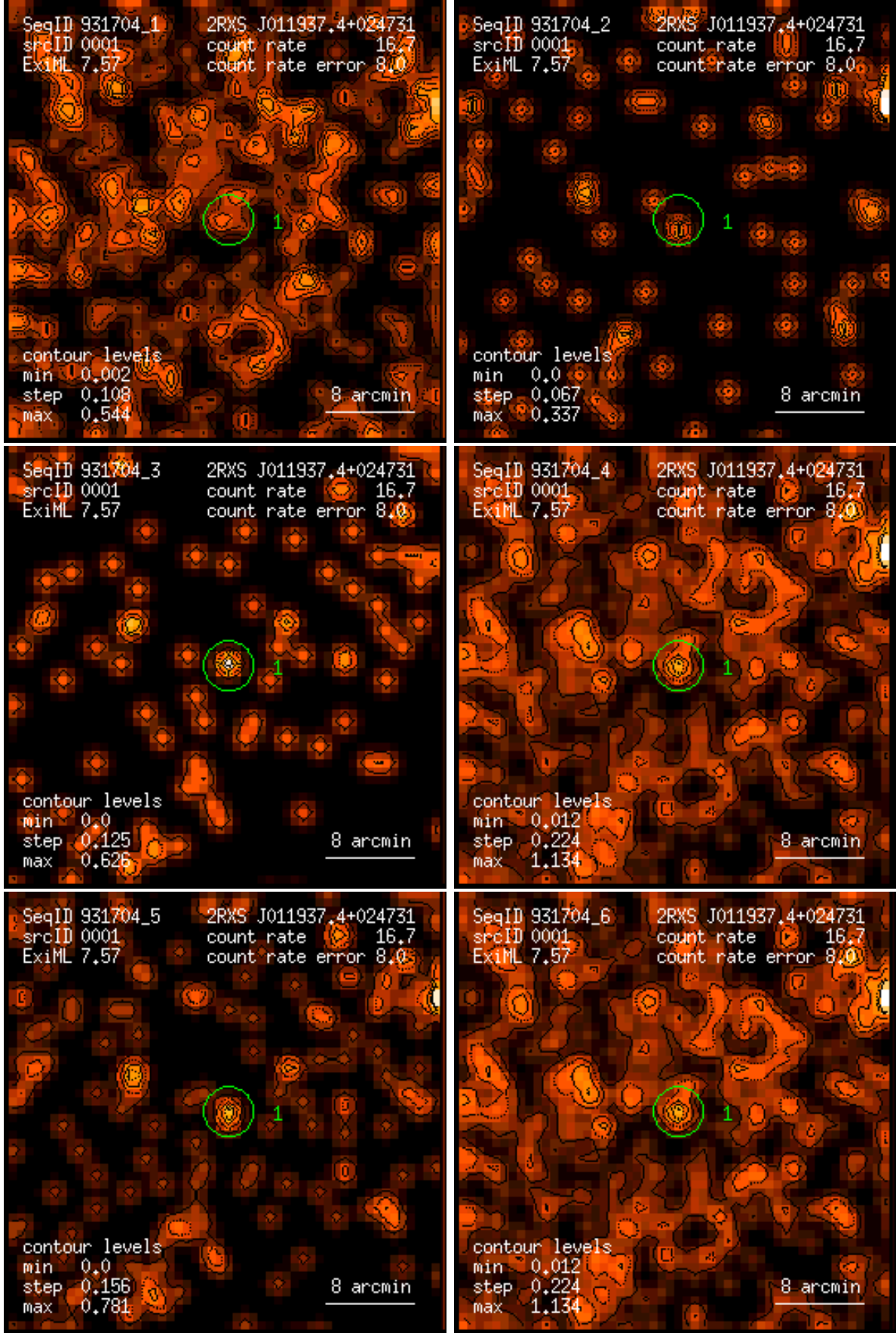
Figure 1: RASS 931704: detection 0001: band rate images, Gaussian filter: (1) PSPC channels 11 – 41, (2) 52 – 90, (3) 91 – 201, (4) 11 – 235, (5) 52 – 201, (6) 11 – 201. Broad band rates in counts/ks. Band rate contour levels in counts/ks/arcmin 2 .
