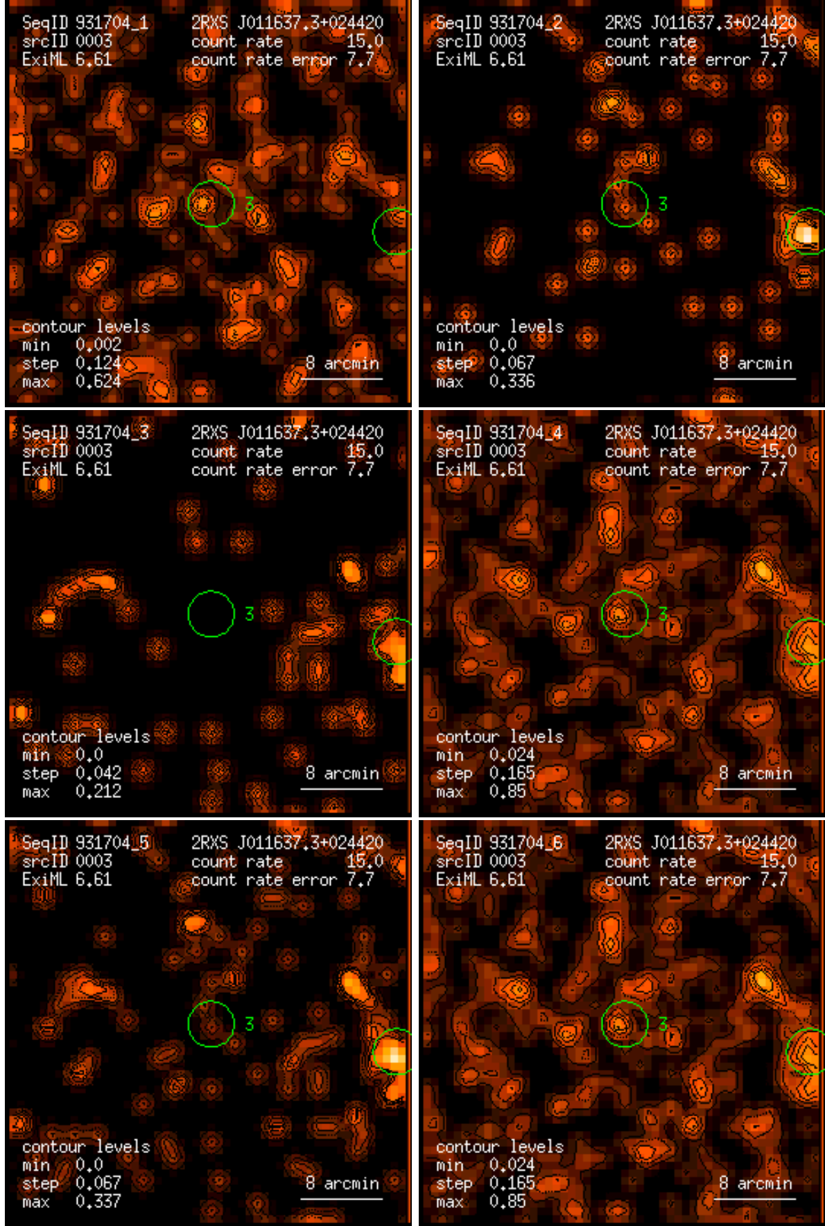
Figure 3: RASS 931704: detection 0003: band rate images, Gaussian filter: (1) PSPC channels 11 – 41, (2) 52 – 90, (3) 91 – 201, (4) 11 – 235, (5) 52 – 201, (6) 11 – 201. Broad band rates in counts/ks. Band rate contour levels in counts/ks/arcmin 2 .
