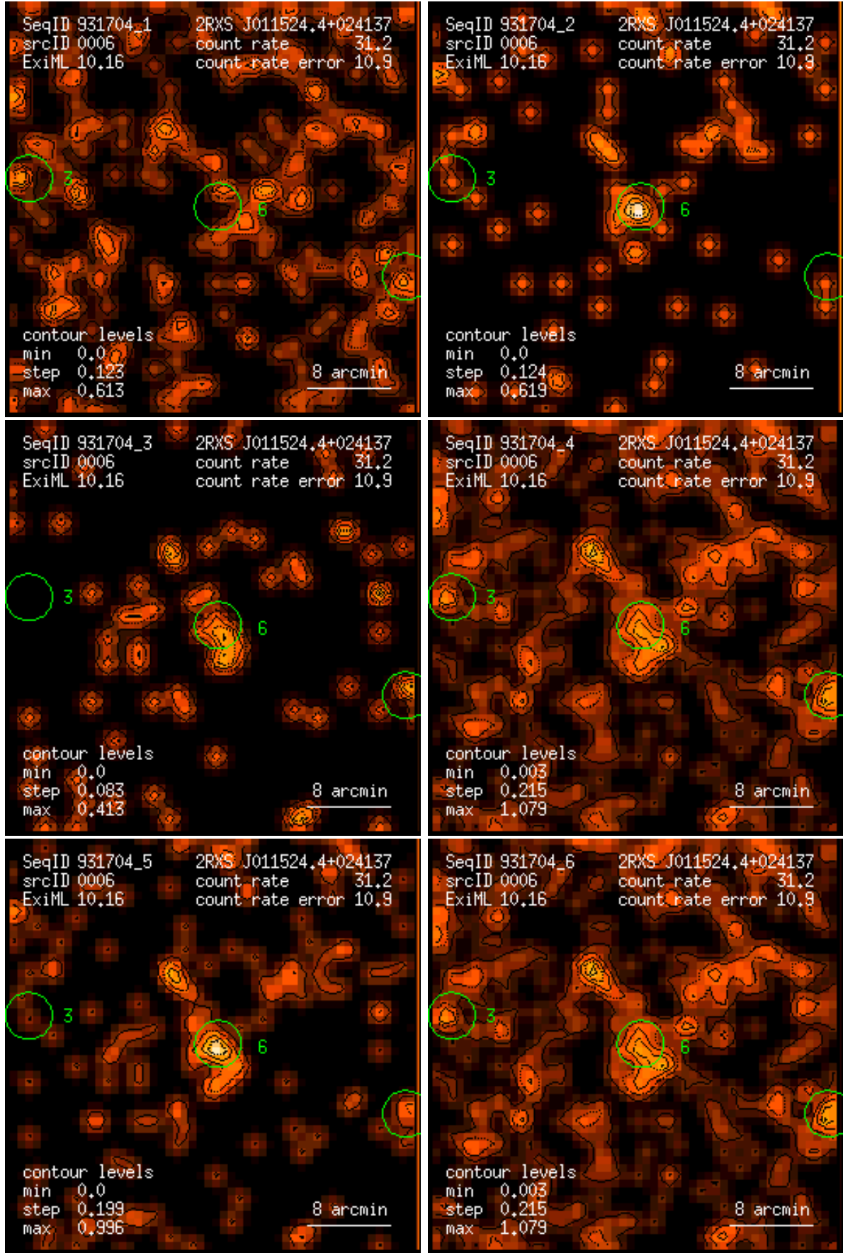
Figure 6: RASS 931704: detection 0006: band rate images, Gaussian filter: (1) PSPC channels 11 – 41, (2) 52 – 90, (3) 91 – 201, (4) 11 – 235, (5) 52 – 201, (6) 11 – 201. Broad band rates in counts/ks. Band rate contour levels in counts/ks/arcmin 2 .
