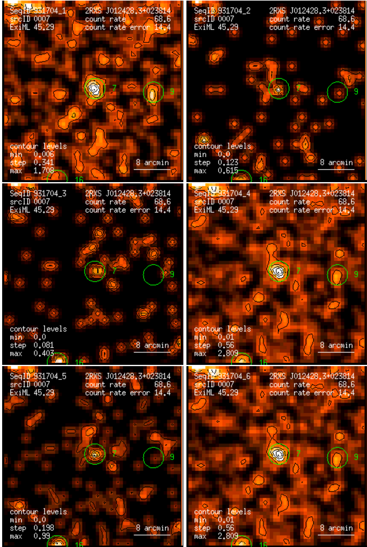
Figure 7: RASS 931704: detection 0007: band rate images, Gaussian filter: (1) PSPC channels 11 – 41, (2) 52 – 90, (3) 91 – 201, (4) 11 – 235, (5) 52 – 201, (6) 11 – 201. Broad band rates in counts/ks. Band rate contour levels in counts/ks/arcmin 2 .
