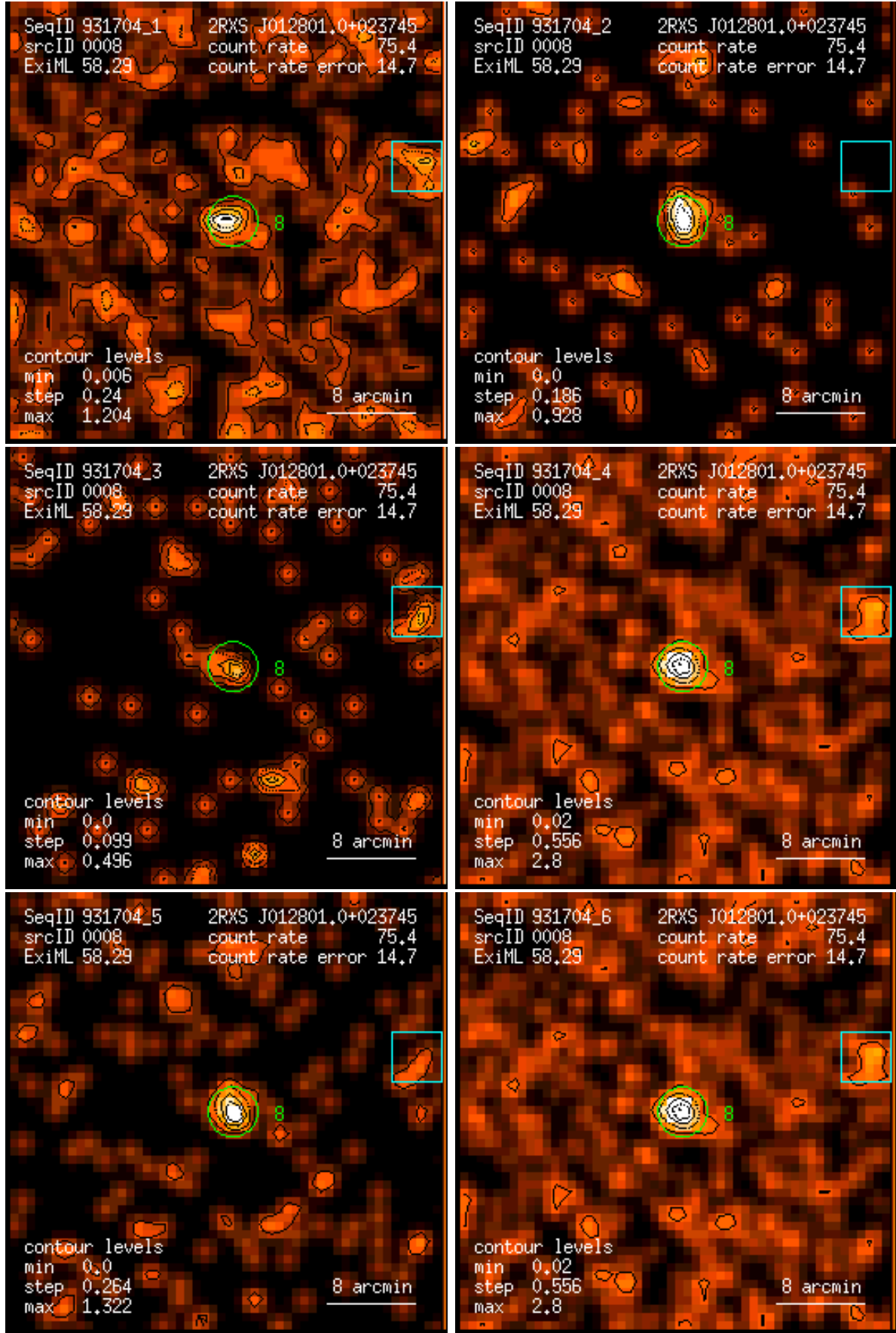
Figure 8: RASS 931704: detection 0008: band rate images, Gaussian filter: (1) PSPC channels 11 – 41, (2) 52 – 90, (3) 91 – 201, (4) 11 – 235, (5) 52 – 201, (6) 11 – 201. Broad band rates in counts/ks. Band rate contour levels in counts/ks/arcmin 2 .
