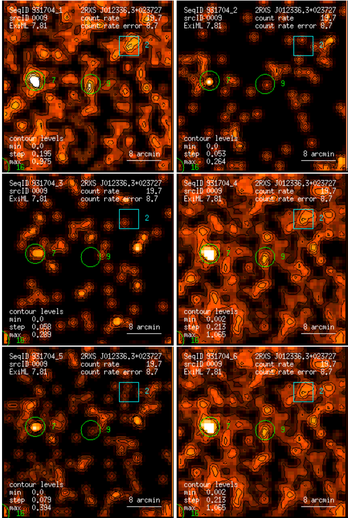
Figure 9: RASS 931704: detection 0009: band rate images, Gaussian filter: (1) PSPC channels 11 – 41, (2) 52 – 90, (3) 91 – 201, (4) 11 – 235, (5) 52 – 201, (6) 11 – 201. Broad band rates in counts/ks. Band rate contour levels in counts/ks/arcmin 2 .
