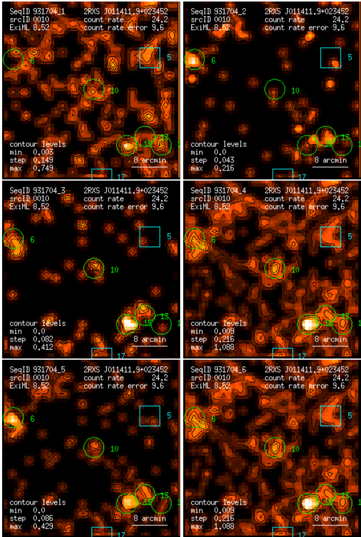
Figure 10: RASS 931704: detection 0010: band rate images, Gaussian filter: (1) PSPC channels 11 – 41, (2) 52 – 90, (3) 91 – 201, (4) 11 – 235, (5) 52 – 201, (6) 11 – 201. Broad band rates in counts/ks. Band rate contour levels in counts/ks/arcmin 2 .
