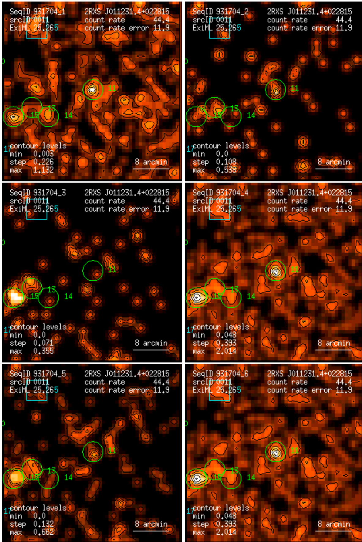
Figure 11: RASS 931704: detection 0011: band rate images, Gaussian filter: (1) PSPC channels 11 – 41, (2) 52 – 90, (3) 91 – 201, (4) 11 – 235, (5) 52 – 201, (6) 11 – 201. Broad band rates in counts/ks. Band rate contour levels in counts/ks/arcmin 2 .
