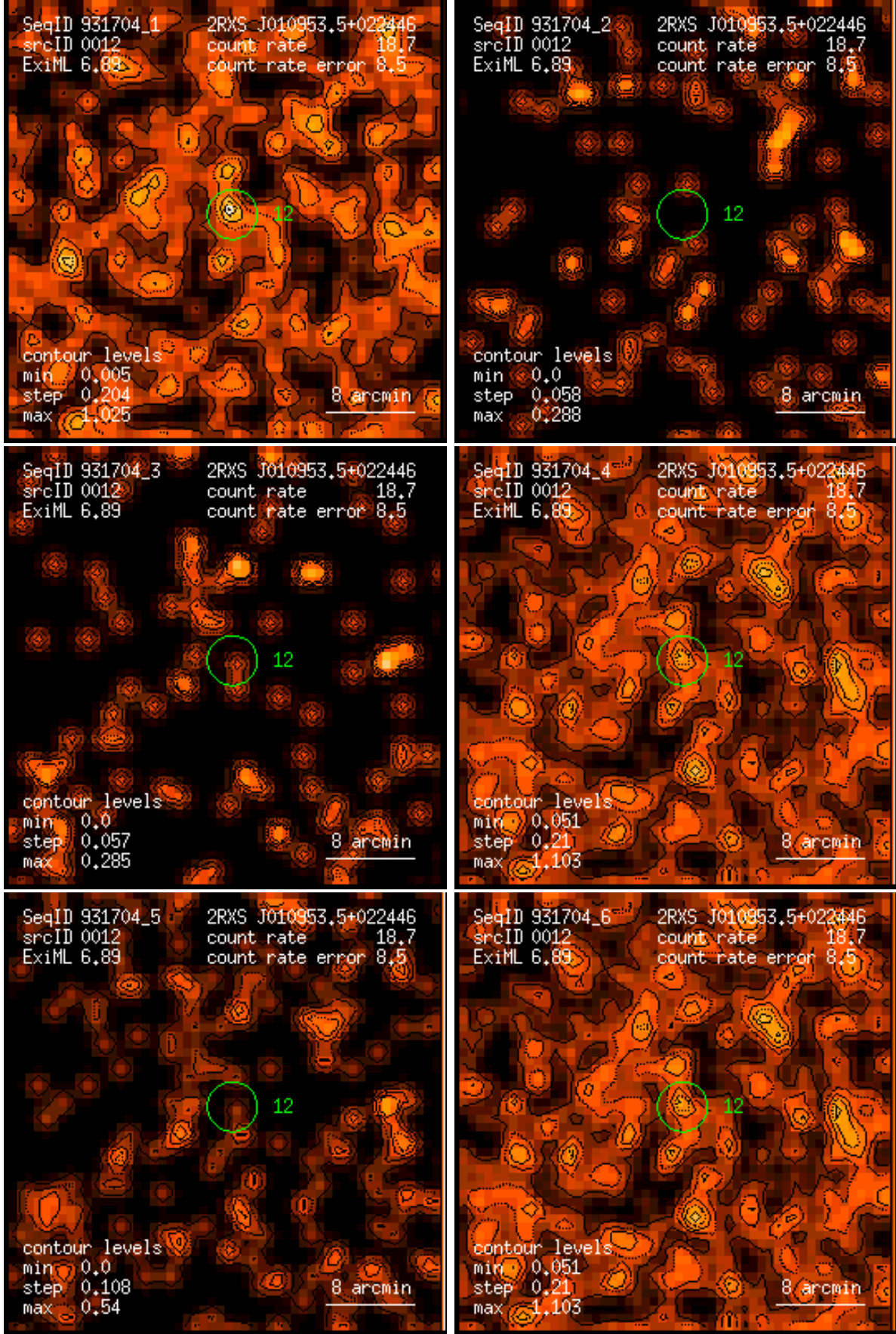
Figure 12: RASS 931704: detection 0012: band rate images, Gaussian filter: (1) PSPC channels 11 – 41, (2) 52 – 90, (3) 91 – 201, (4) 11 – 235, (5) 52 – 201, (6) 11 – 201. Broad band rates in counts/ks. Band rate contour levels in counts/ks/arcmin 2 .
